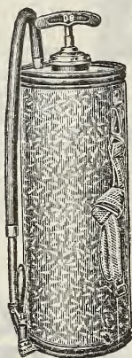
Compressed Air Sprayer No. 15.
