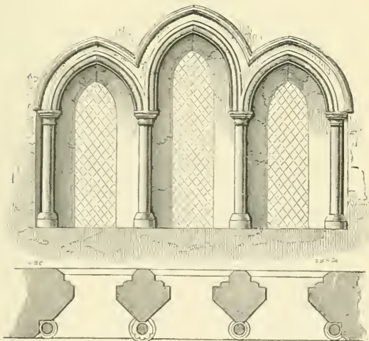
120. Window at the west end of the Hall of the King's Palace at Winchester, A.D. 1222—1235.
