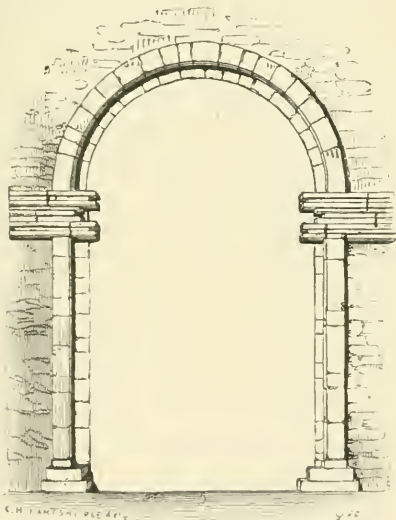
8. Barnack b , Northamptonshire. Tower-arch of Anglo-Saxon character.
