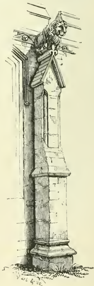
146. Over, Cambridgeshire. Buttress, with set-off and pediment, or gablet, with the angles of the upper stage chamfered.
