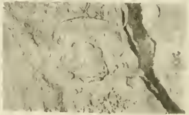
ORIGINAL COLLECTION OF CAMBRIAN TRILOBITES FROM SONORA (See explanation of plates at end of text.)
