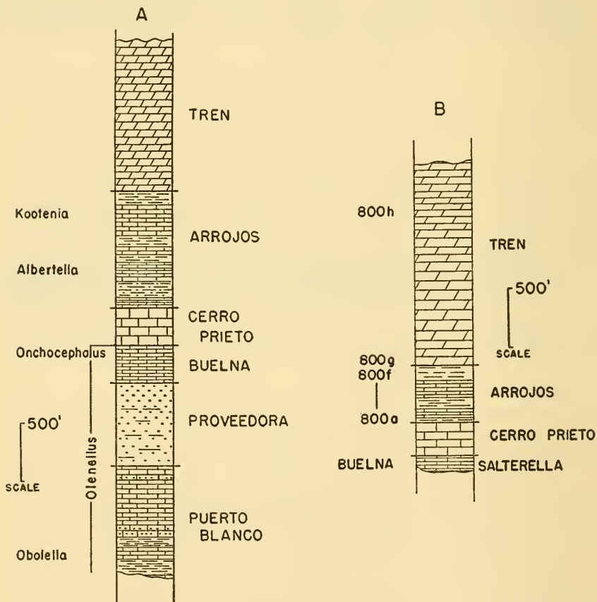
FIG. 6.—Columnar sections of Proveedora Hills (A) and Arrojitos Hills (B) showing formations. Differences in thickness between the sections are clearly shown.
