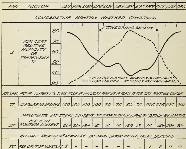
FIG. 7.—Graphic air-seasoning chart for the Inland Empire
