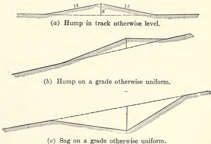
FIG. 25.—Sags and humps on grades otherwise uniform.
