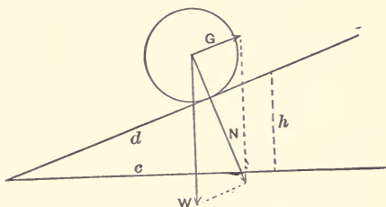
FIG. 23.—Grade resistance.
