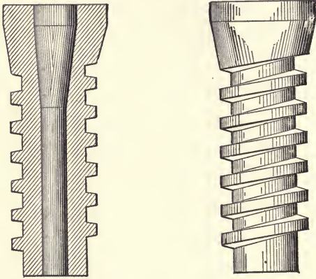
FIG. 22.—Wooden dowels for ties.
