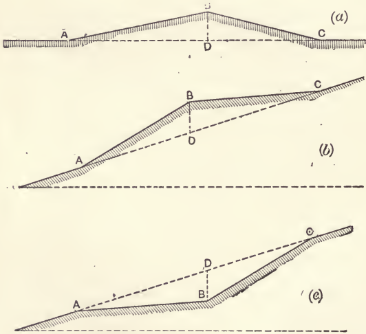
FIG. 34.—Types of "rise and fall".
