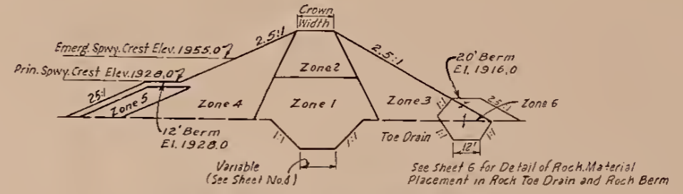
TYPICAL SECTION - ZONED EMBANKMENT
