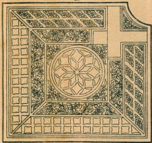
裏櫺外轉角平棊
