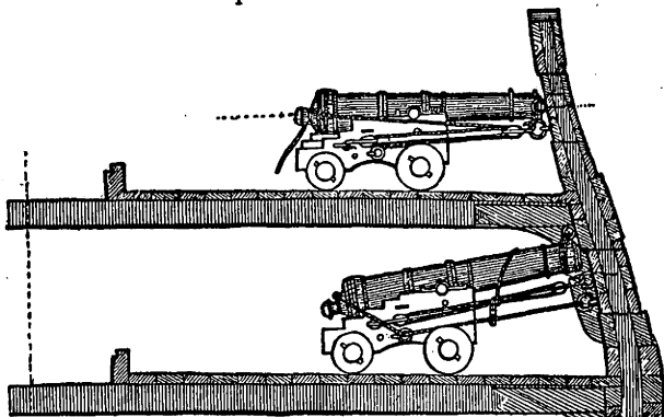
Guns Secured for a Gale. From the "Kedge Anchor."
