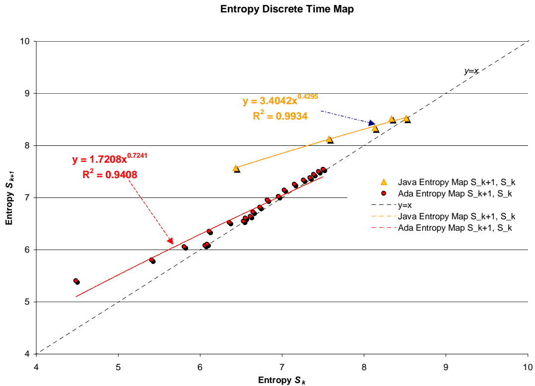
Figure III-23 Java and Ada State Space Finite Difference Map S_{k+1}, S_k
