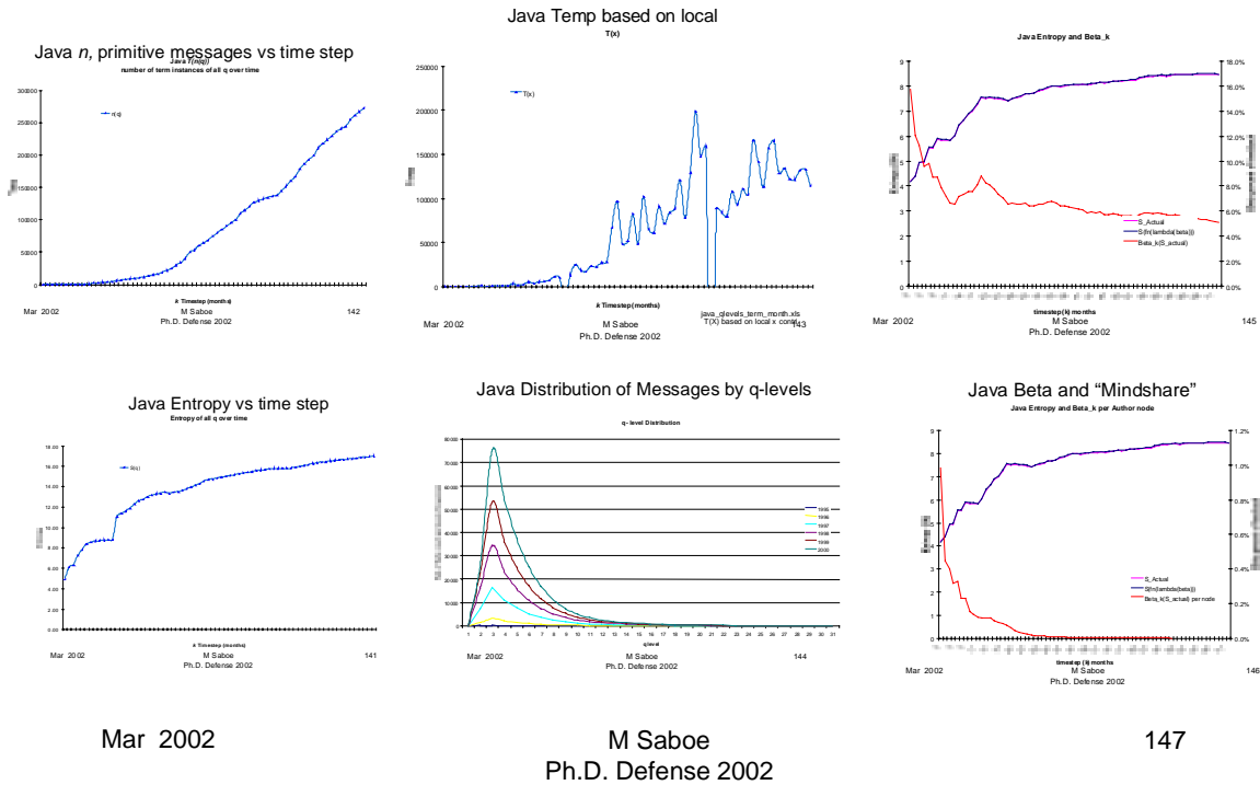
Figure IV-15 Java Relationships
