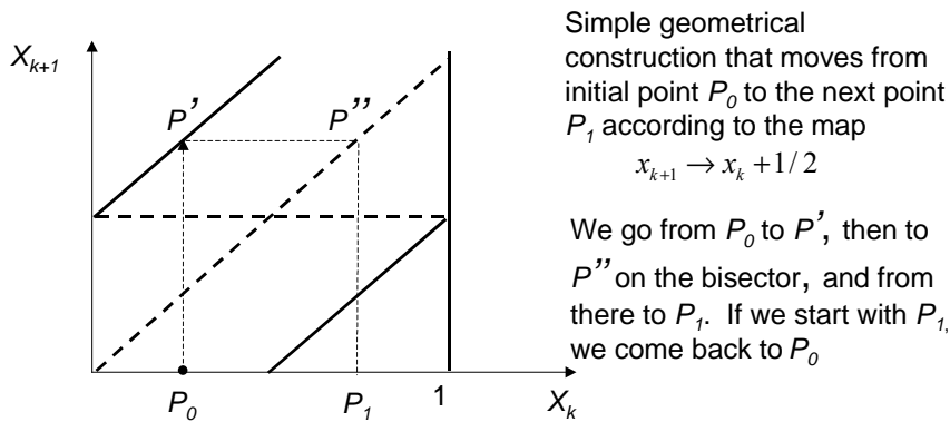
Figure A-5 Periodic Map (Source: Prigogine 1997, p82)
