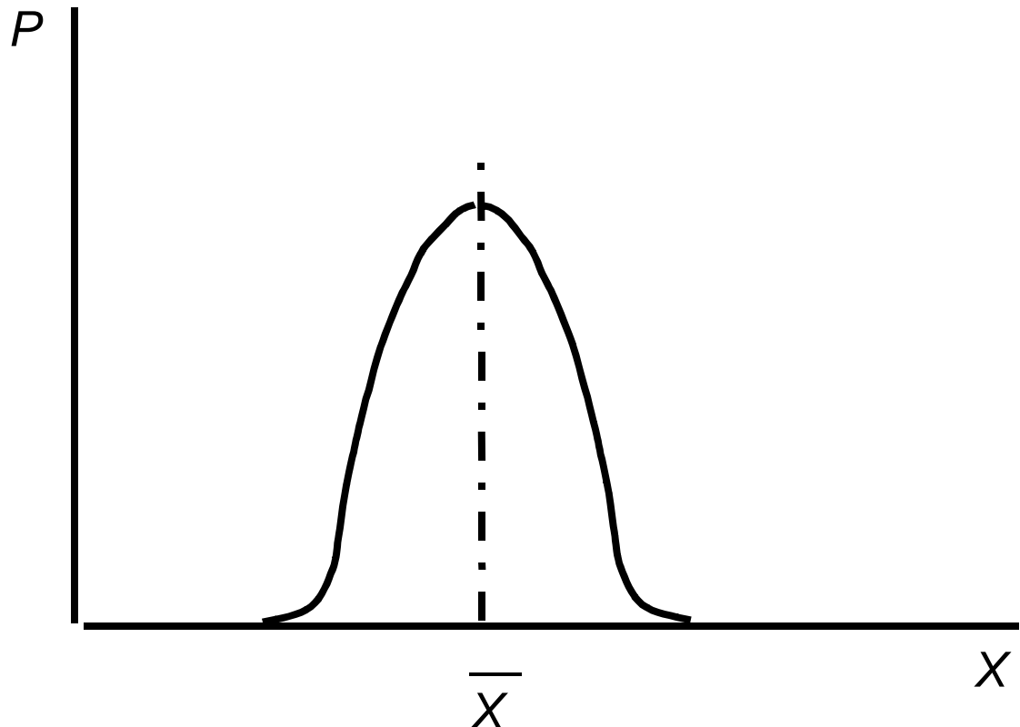
Figure A-9 Uni-modal Distribution
