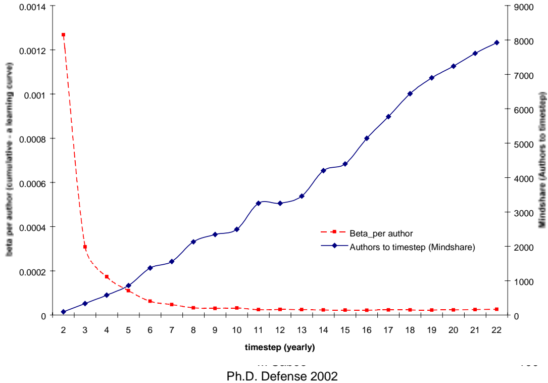
Figure IV-18 \beta Feedback requested from persistent messages, allocated per author.
