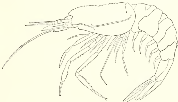
FIG. 7. Parapasiphæa serrata . ♀ ( \times about 1½). Station 2919.
