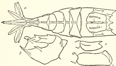
FIG. 69. Crangon variabilis . ♀. Station 2842. a. Dorsal view of carapace and abdomen (×2). b. Side view of carapace (×2). c. Acicula (×4). d. Chela (×4).
