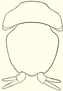
FIG. 104. Last thoracic segment, abdomen, and uropoda ( \times 41 ).
