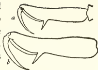
FIG. 61. Crangon franciscorum ( \times 2\frac{1}{2} ). a. Chela of ♂. San Francisco market. b. Chela of ♀. Station 2528.
