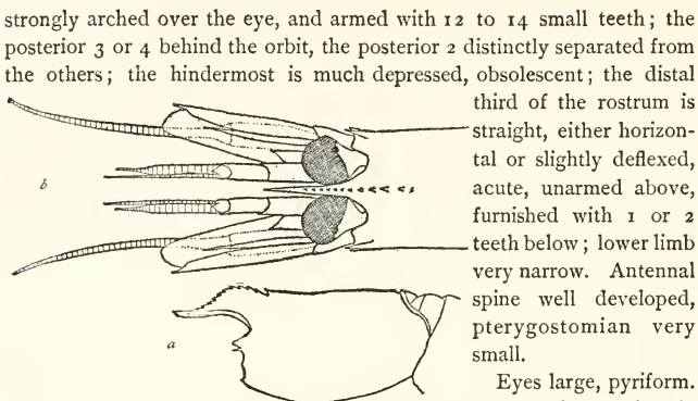
FIG. 47. Spirentocaris avina . Station 2853. a. Side of carapace ( \times 3 ). b. Dorsal view of anterior portion ( \times 4 ).
