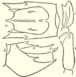
FIG. 68. Crangon acclivis . a. Dorsal view of carapace, ♂ (×4). Station 2948. b. Side view (×3½). c. Acicula, ♀ (×8). d. Chela, ♀ (×8).
