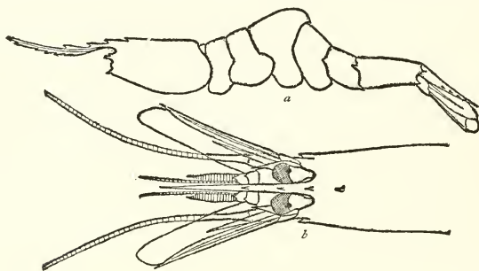
FIG. 32. Spirontocaris flexa . \varphi . Station 2850. a . Side of carapace and abdomen ( \times 2 ). b . Dorsal view of anterior portion ( \times 3 ).
