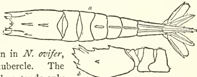
FIG. 80. Nectocrangon californiensis (× 2). Station 3664. a. Dorsal view of carapace and abdomen. b. Side view.
