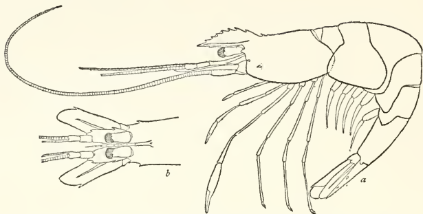
FIG. 10. Urocaris infraspinis . ♀ ( \times 34 ). Locality unknown. a. Side. b. Dorsal view of anterior portion.
