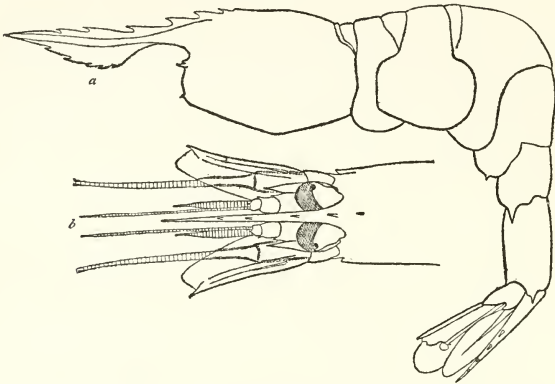
FIG. 38. Spiontocaris suckleyi . ♀ ( \times 2\frac{1}{2} ). Station 3334. a. Side. b. Dorsal view of anterior portion.
