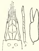
FIG. 49. Betseus harrimani . a. Dorsal view of anterior portion ( \times 4 ). b. Carpus and chela of second pair ( \times 5\frac{1}{2} ). c. Left chela of first pair ( \times 2\frac{1}{2} ).
