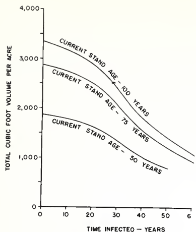
Figure D-5. — Total cubic-foot volume per acre in 50-, 75-, and 100-year-old lodgepole pine stands in relation to length of time dwarfmistletoe has been present.
