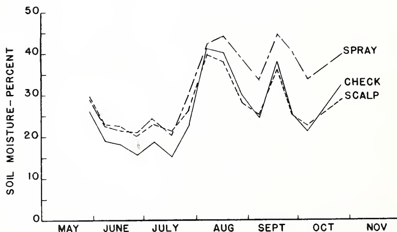
PERCENT SOIL MOISTURE AT 0-8 INCH DEPTH AT WING MOUNTAIN IN 1961
