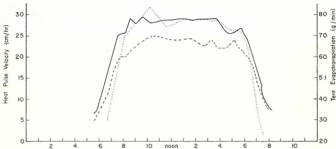
Figure W-15. — Comparison of relative sap velocity and transpiration measured by the tent method for an alligator juniper tree 12 feet tall. The solid line indicates heat-pulse velocity measured at a height of 5 feet in the stem, while the dashed line indicates heat-pulse velocity at a height of 0.5 foot. The dotted line indicates evaporation measured by the tent method. The close correlation of the two methods is evident.
