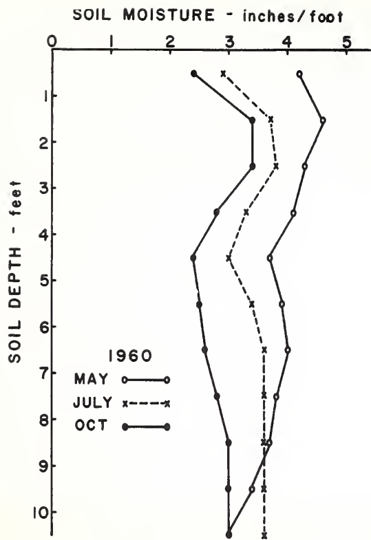
Figure F-1. — Soil-moisture measurements under a 20-year-old windbreak to a depth of 11 feet show water depletion as the 1960 growing season progressed. Seward County, Nebraska.
