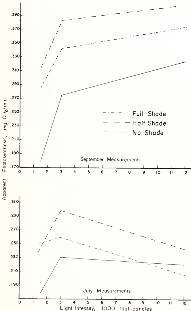
Figure F-12. — Apparent photosynthesis of individual Engelmann spruce seedlings grown under full shade, half shade, and no shade, when exposed to light intensities of 1,500, 3,000, and 12,000 foot-candles.
