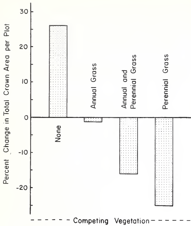
Figure R-1. — Changes in crown cover of burweed from June to November 1961 when grown alone and when competing with other plants (Santa Rita Experimental Range).
