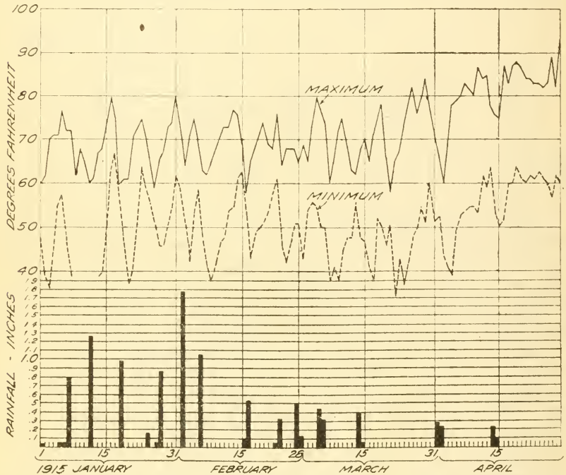
FIG. 2.—Precipitation and maximum and minimum temperatures at Orlando, Fla., during January, February, March, and April, 1915—a year of severe scab infection.
