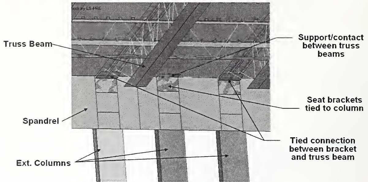
Figure 3-15. Truss floor connection detail at exterior wall.
