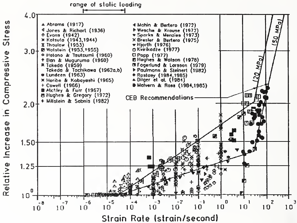
Source: From "Compressive behavior of concrete at high strain rates," published in Mater. Struct. 24 (1991) Courtesy RILEM.
