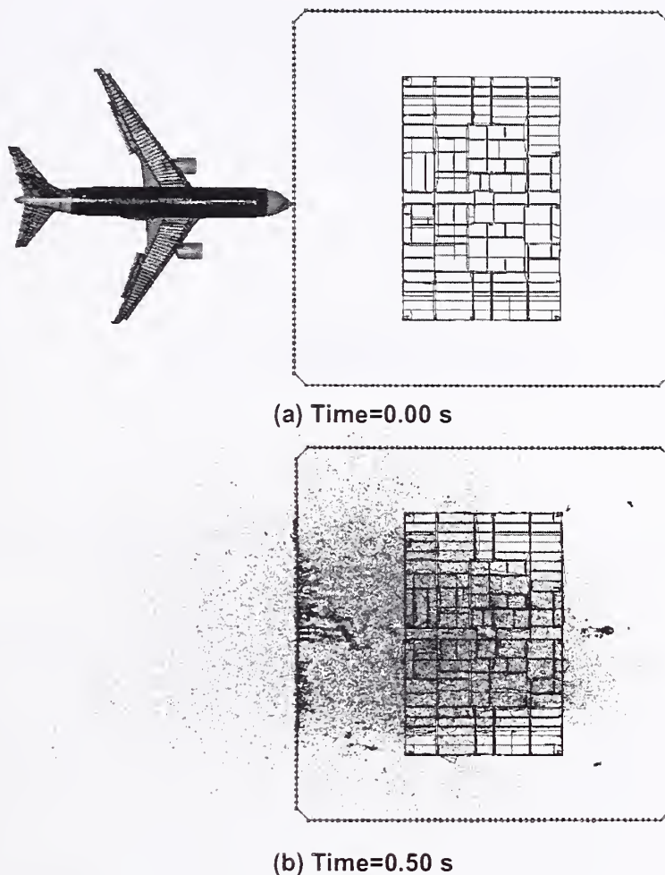
Figure E-26. WTC 1 base case global impact analysis – top view.
