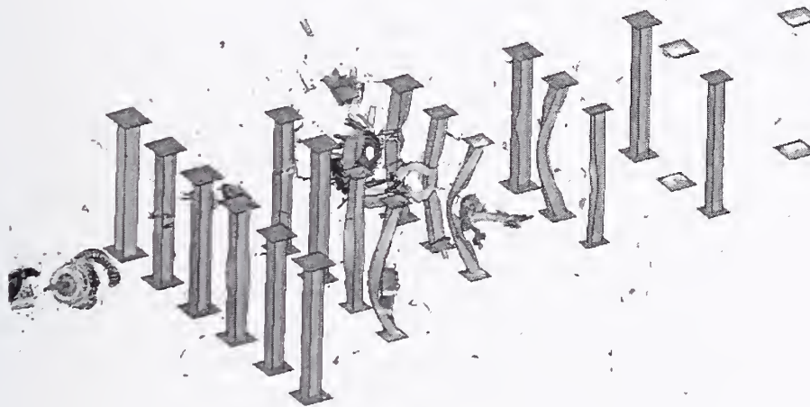
(b) Impact response at 0.20 s
