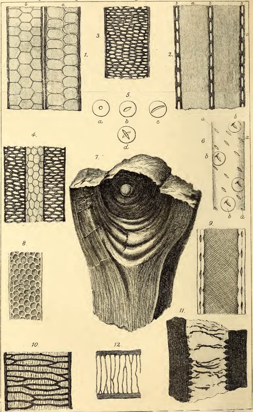
Exogenous Stems from Coal-Measures.
