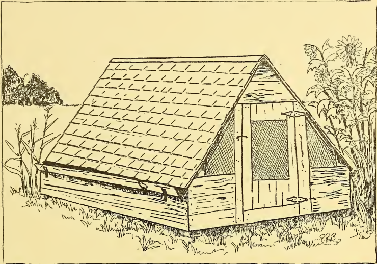
Colony house to accommodate from 12 to 25 fowls. This house is eight feet square on the ground and eight feet from floor to apex of roof. There is no frame, but the roof boards are nailed to the ridgepole and to plank baseboards.
