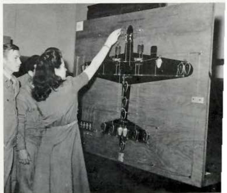
Mockup, Arrangement of Lighting, Ground, Relay, etc., to Show How to Trace Circuits.
