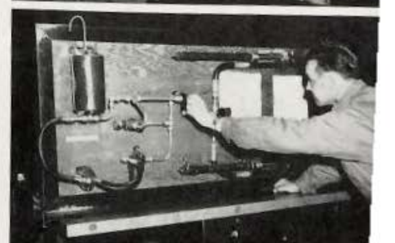
Mockup, Gun Charging System.
