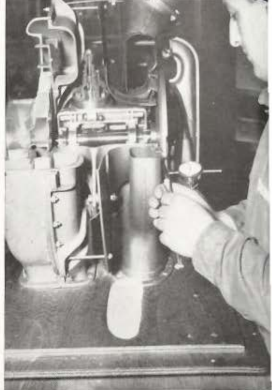
Cutaway, Turbo Supercharger.
