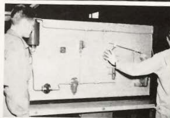
Mockup, Pressure Reducing Valve System.
