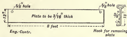
Fig. 45.—Form for Applying Cement Facing (Massachusetts Highway Commission).
