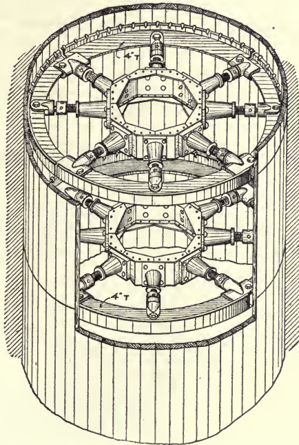
Fig. 54.—Curbing for Concrete Piers (Jackson Patent).
