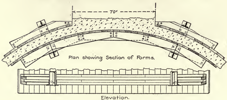
Fig. 287.—Forms for Constructing Grain Elevator Bins.
