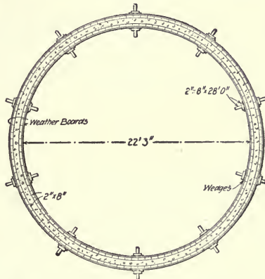
Fig. 286.—Form for Constructing Silo.
