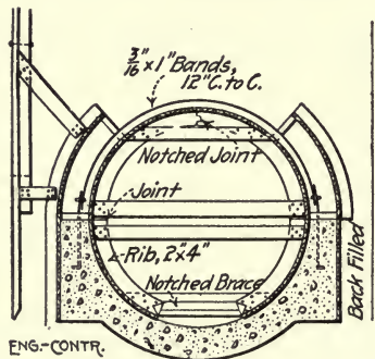
Fig. 259.—Form for South Bend Sewer (Third Stage).
