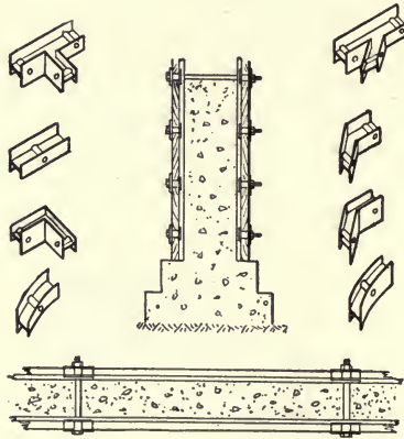
Fig. 206.—Farrell's Plank Holders for Wall Forms.
