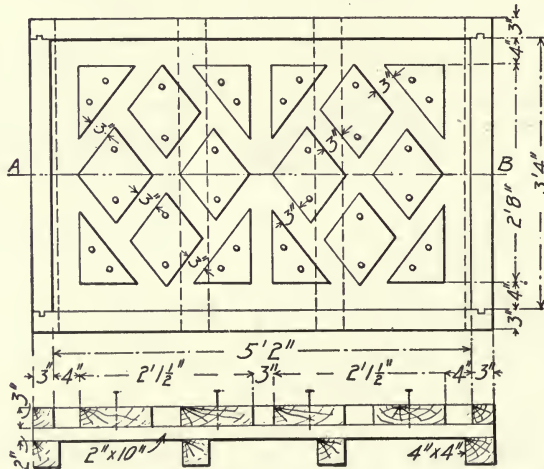
Fig. 291.—Form for Lattice Panels Shown by Fig. 290.
