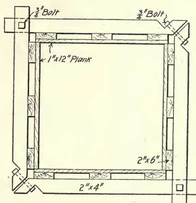
Fig. 184.—Form for Large Rectangular Columns.
