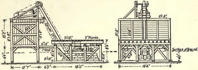
Fig. 73.—Stone Crushing Plant for Lock Walls, Illinois & Mississippi Canal. sides of the pit were tracks from the sand and stone piles and on the other two sides were the cement platform and water tank. The charging box dumped into the hopper above the mixer and the mixer discharged into cars underneath. A 15-HP. engine operated the hoist by one pulley and the mixer by the other pulley. Nine revolutions of the mixer made a
