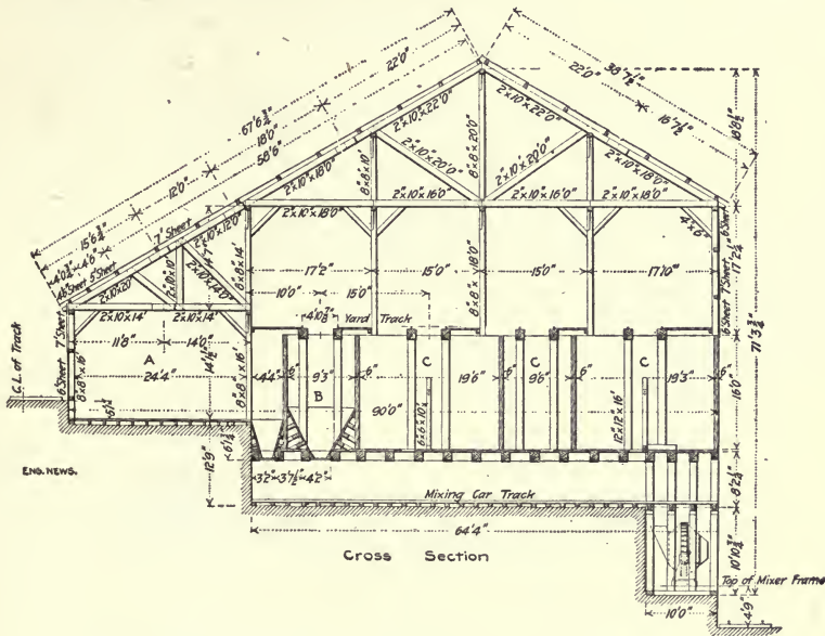
Fig. 91.—Concrete Mixing Plant for McCall Ferry Dam.
