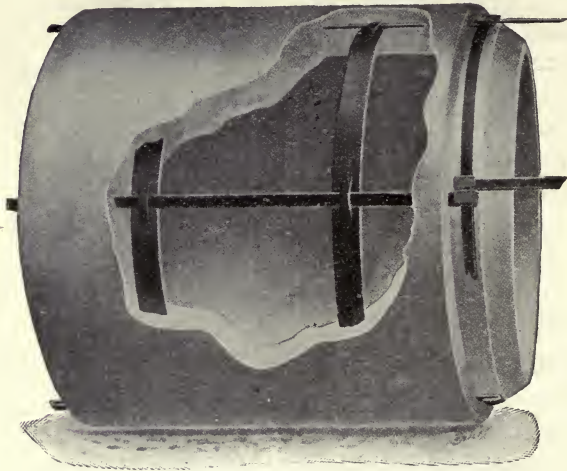
Fig. 269.—Jackson Concrete Sewer Pipe.
