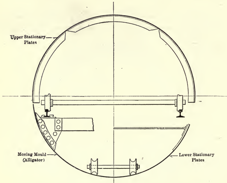
Fig. 252.—Traveling Form for Pinto Creek Conduit.
