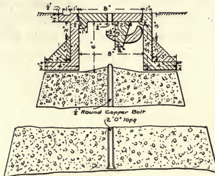
Fig. 304.—Bench Monument, Chicago, Ill.
