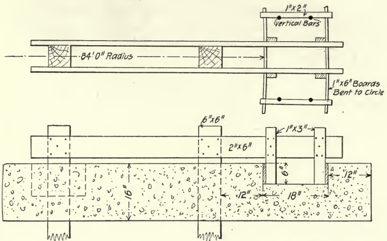
Fig. 280.—Forms for Constructing Channel for Wall in Reservoir Floor.
