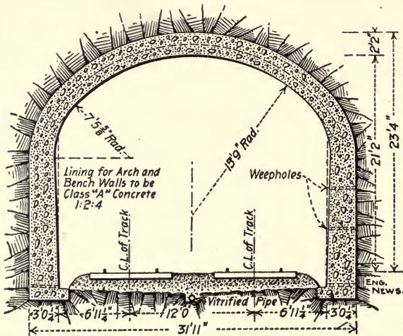
Fig. 131.—Cross-Section of Peekskill Tunnel, Showing Lining.
