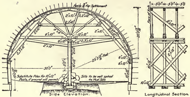
Fig. 148.—Center for 50 ft. Arch Span (Supported).
