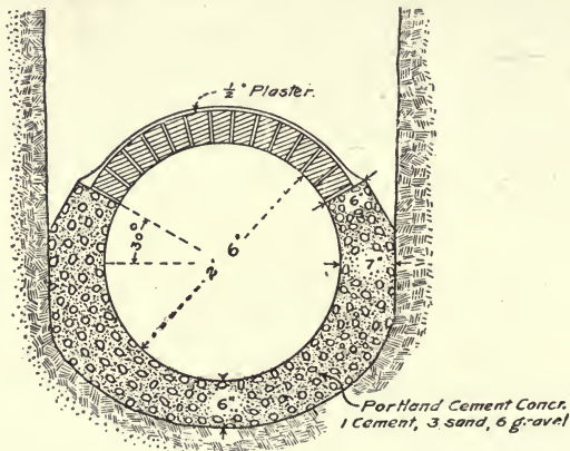
Fig. 266.—Sewer with Monolithic Invert and Block Arch.
