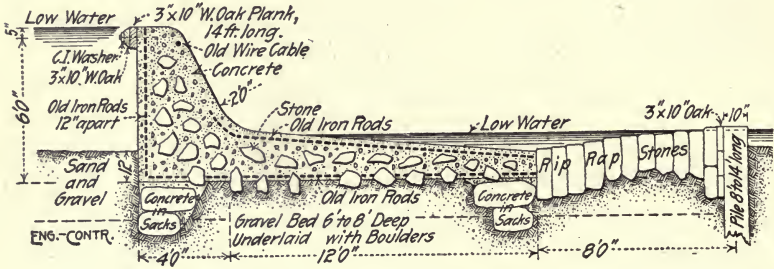
Fig. 89.—Concrete Dam at Richmond, Ind.
