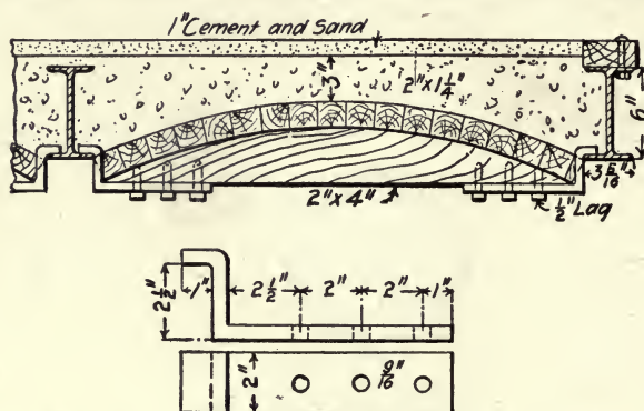
Fig. 192.—Form for Arch Slab Between I-Beams.
