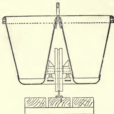
Fig. 18.—Charging Bucket With Wheel and Detachable Handle.
