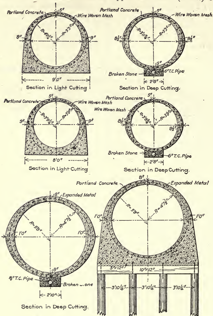
Fig. 265.—Cross-Sections of Sewer at Wilmington, Del.
