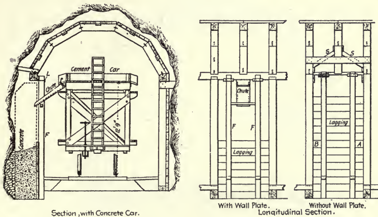
Fig. 130.—Sketches Showing Method of Lining Mullan Tunnel.
