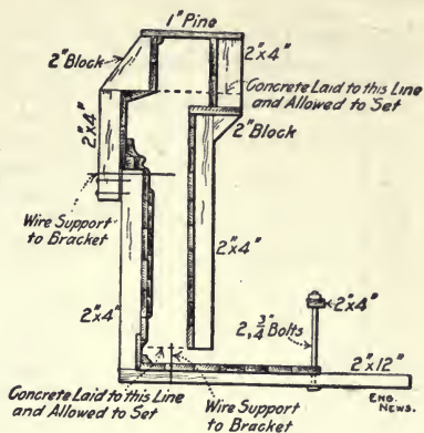
Fig. 297.—Form for Concrete Facade Shown by Fig. 298.
