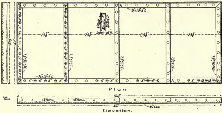
Fig. 128.—Steel Forms for Side Walls for Capitol Hill Tunnel.
