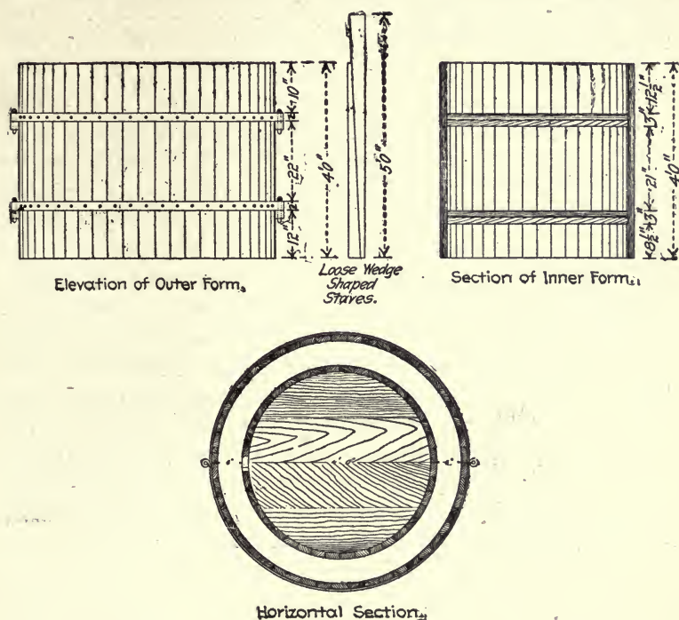
Fig. 176.—Form for Molding Culvert Pipe.
