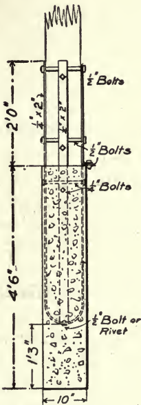
Fig. 305.—Base for Wooden Pole.
