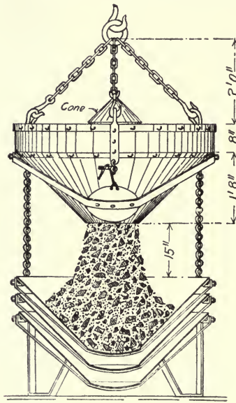
Fig. 25.—Hains Gravity Mixer, Telescoping Hopper Form.
