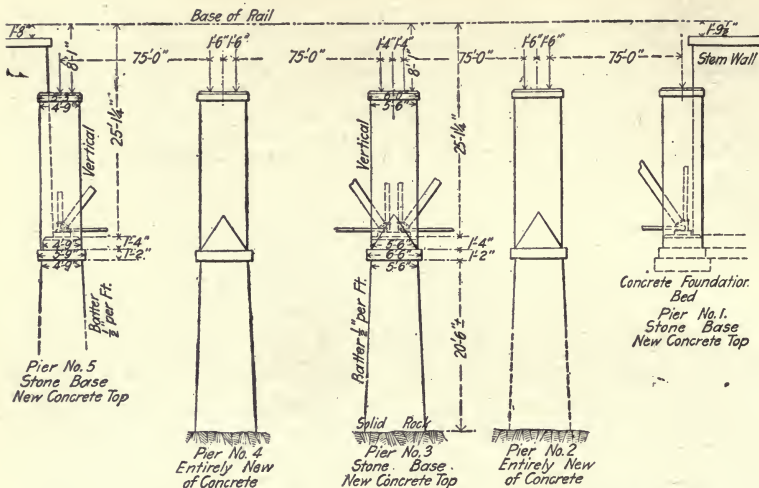
Fig. 94.—Diagram Arrangement of Piers, Calf Killer River Bridge.
