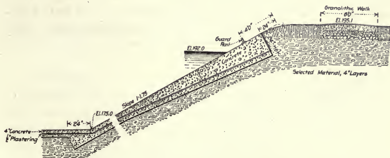
Fig. 285.—Section of Reservoir Lining, Quincy, Mass.
