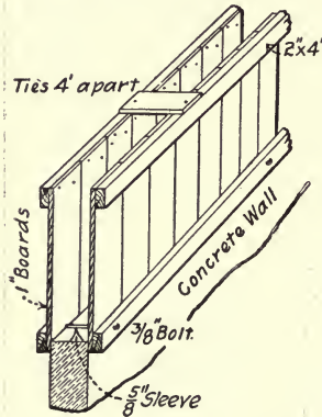
Fig. 203.—Sectional Form for Wall Construction.
