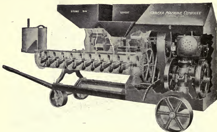
Fig. 22.—Eureka Automatic Feed Continuous Mixer.
