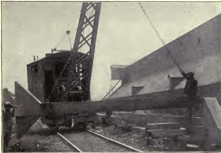
Fig. 243.—View Showing Method of Hoisting Molded Columns.
