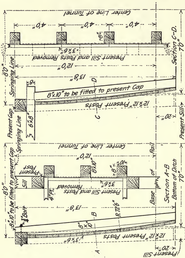
Fig. 135.—Side Wall Forms for Plans A and B, Fig. 134.
