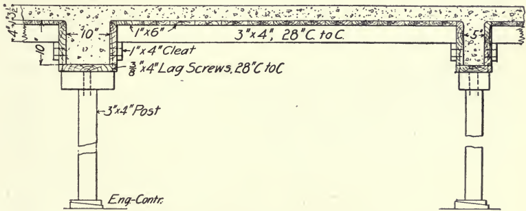
Fig. 227.—Girder and Slab Forms for 6-Story Building.
