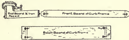
Fig. 121.—Box Form for Concrete Curb.
