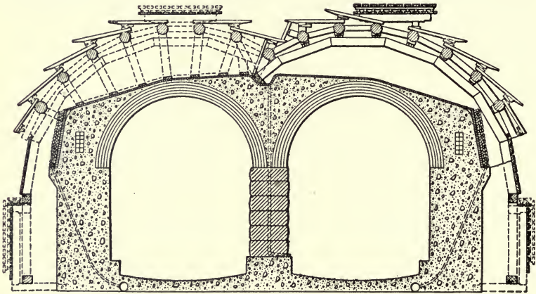
Fig. 126.—Section Showing Lining for Capitol Hill Tunnel, Washington, D. C.
