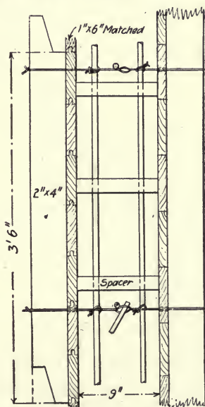
Fig. 202.—Sectional Form for Wall Construction.
