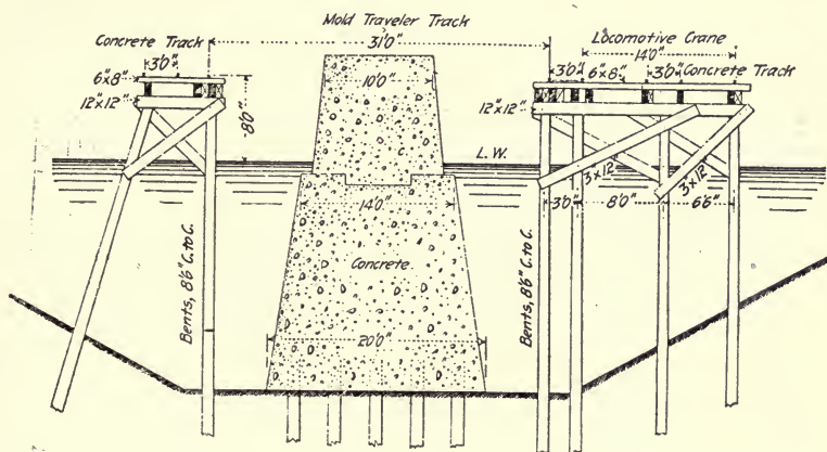
Fig. 85.—Cross-Section of Concrete Pier, Superior, Wis.
