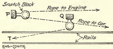
Fig. 165.—General Plan of Rope Haulage System.
