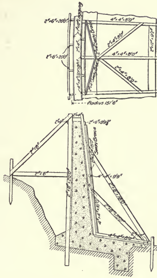
Fig. 278.—Reservoir Forms, Bloomington, Ill.
