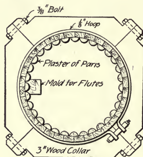
Fig. 190.—Form for Molding Fluted Cylindrical Column.
