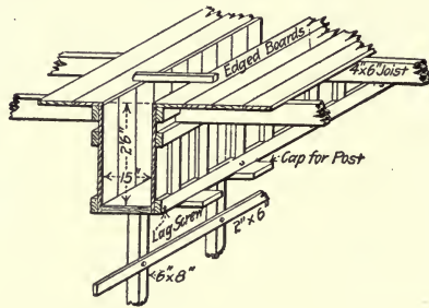
Fig. 199.—Girder and Slab Form for Factory Building, New York, N. Y.
