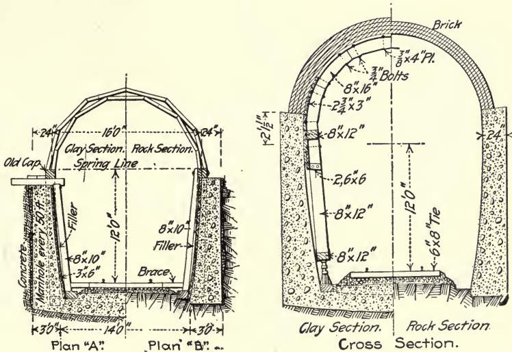
Fig. 136.—General Plan of Centers for Roof Arch, Hodges' Pass Tunnel.
