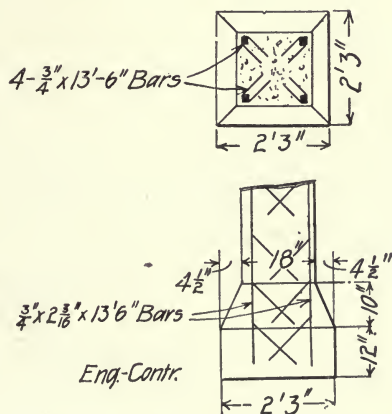
Fig. 276.—Column Construction for 75,000-Gallon Reservoir.
