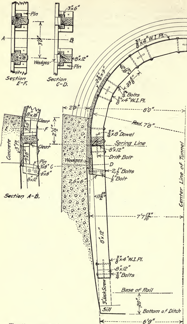
Fig. 137.—Details of Centers for Roof Arch, Hodges' Pass Tunnel.
