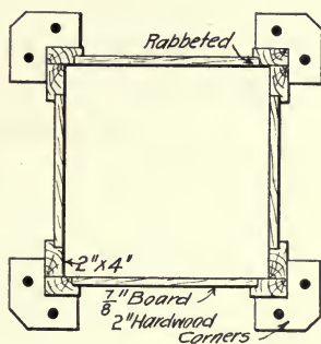
Fig. 177.—Form for Rectangular Column for Factory Building, Cincinnati, O. gineers to a greater extent now than formerly. It is a time consuming method and with wet mixtures it has nothing to recommend it. For lagging 1\frac{1}{4} and 2-in. plank are commonly used; with yokes spaced 2 ft. apart the lighter plank is amply strong and reduces the weight of the units to be handled as well as the amount of form lumber required.
