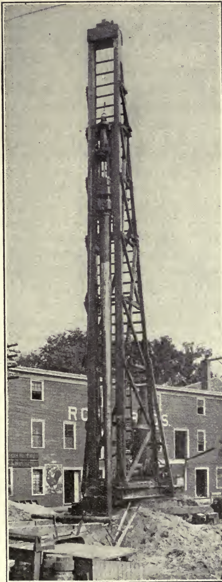
Fig. 49.—Pile Driver Rigged for Constructing Raymond Concrete Piles.
