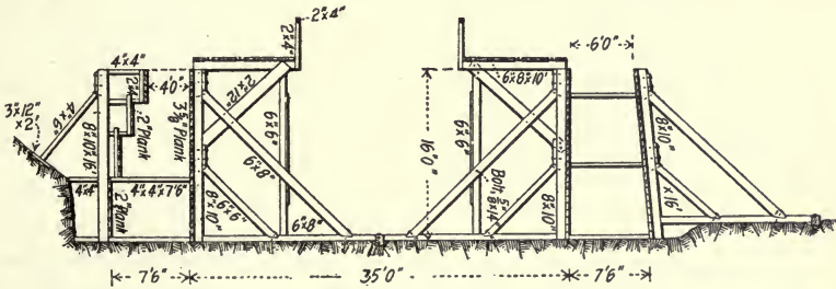
Fig. 74.—Forms for Guard Lock, Illinois & Mississippi Canal.
