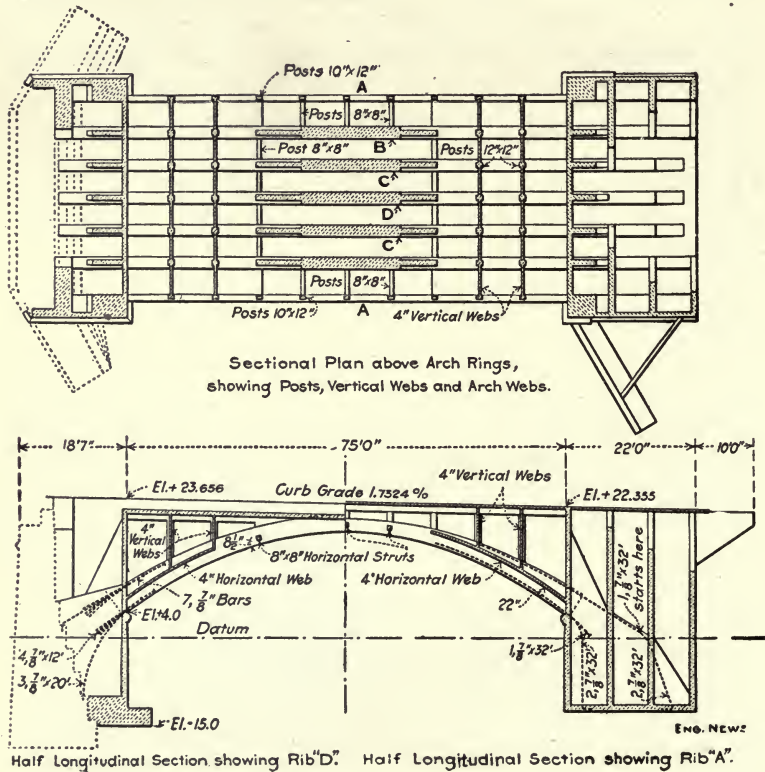
Fig. 168.—Details of Ribbed Arch Bridge.
