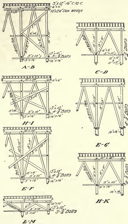
Fig. 158.—Center for Connecticut Ave. Bridge (Details).
