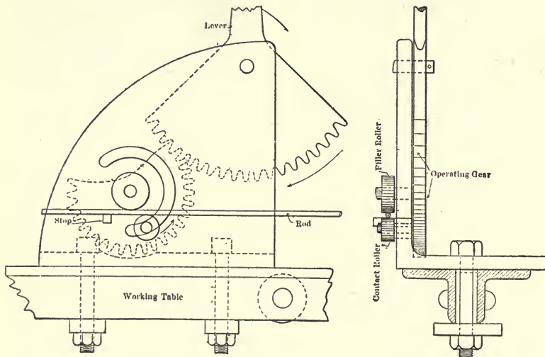
Fig. 212.—Device for Bending Reinforcing Rods.
