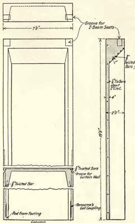
Fig. 228.—Channel Section Wall Column for Factory Building.
