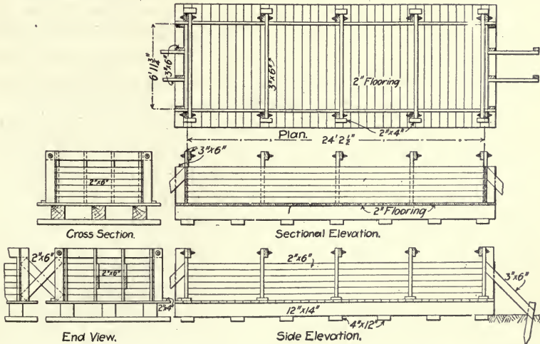
Fig. 156.—Form for Molding Slabs for Girder Bridge.
