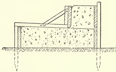
Fig. 122.—Continuous Form for Concrete Curb.
