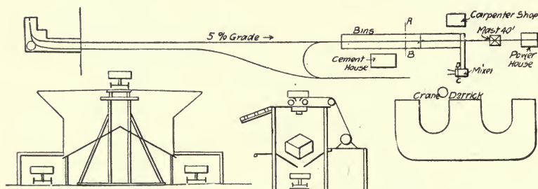
Fig. 69.—Sketch Plans of Concrete Making Plant for Battery Emplacement.
