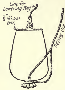
Fig. 31.—Bag for Depositing Concrete Under Water.
