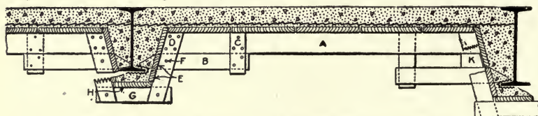
Fig. 193.—Form for Flat Slab Floor Between I-Beams.
