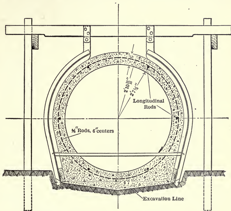
Fig. 251.—Cross-Section of Pinto Creek Irrigation Conduit.
