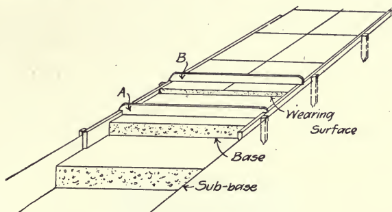
Fig. 116.—Sketch Showing Method of Constructing Cement Walks.
