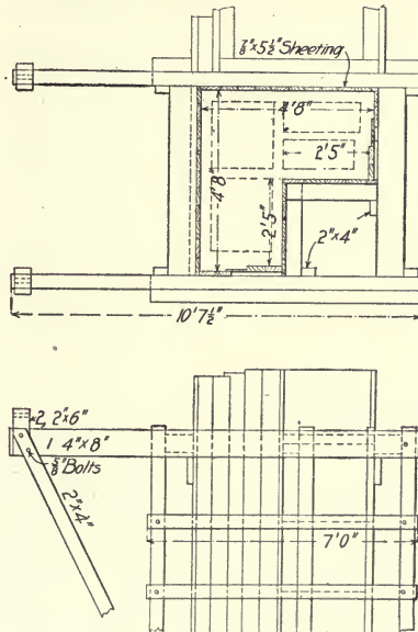
Fig. 182.—Form for Corner Wall Column.
