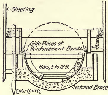
Fig. 258.—Form for South Bend Sewer (Second Stage).
