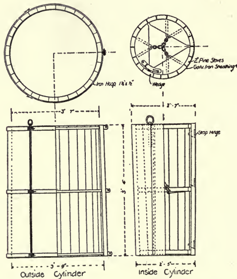
Fig. 250.—Form for Circular Catch Basin or Manhole.
