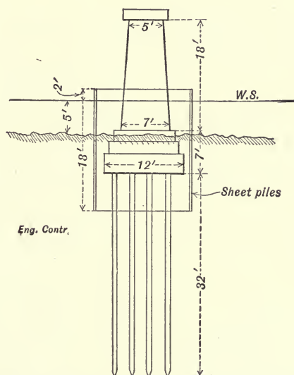
Fig. 93.—Pier and Cofferdam for a Railway Bridge.
