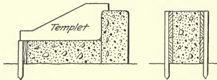
Fig. 124.—Form for Two-Piece Curb Construction.
