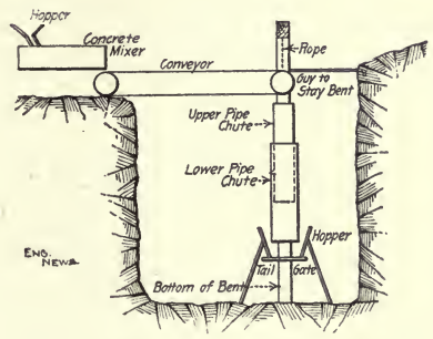
Fig. 14.—Belt Conveyor and Chute for Handling Concrete.
