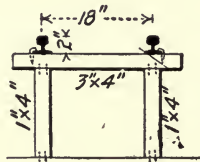
Fig. 162.—Trestle for Service Track.
