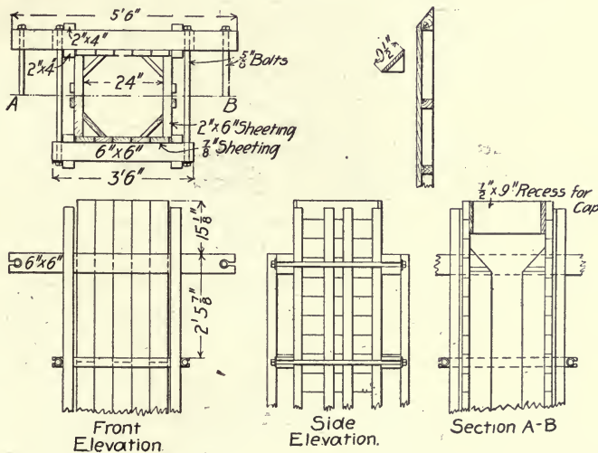
Fig. 186.—Form for Octagonal Column for a Factory Building.
