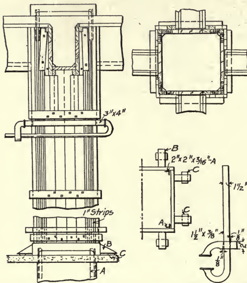
Fig. 185.—Adjustable Form for Rectangular Columns.
