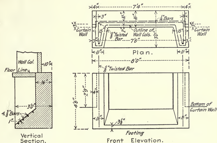
Fig. 229.—Footing for Wall Column Shown by Fig. 228.
