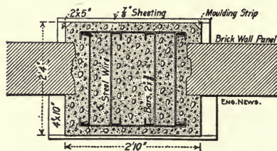
Fig. 223.—Section of Rectangular Wall Column.
