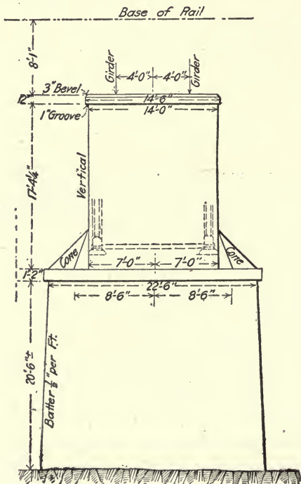
Plan and Elevation of Piers 2, 3 and 4.
