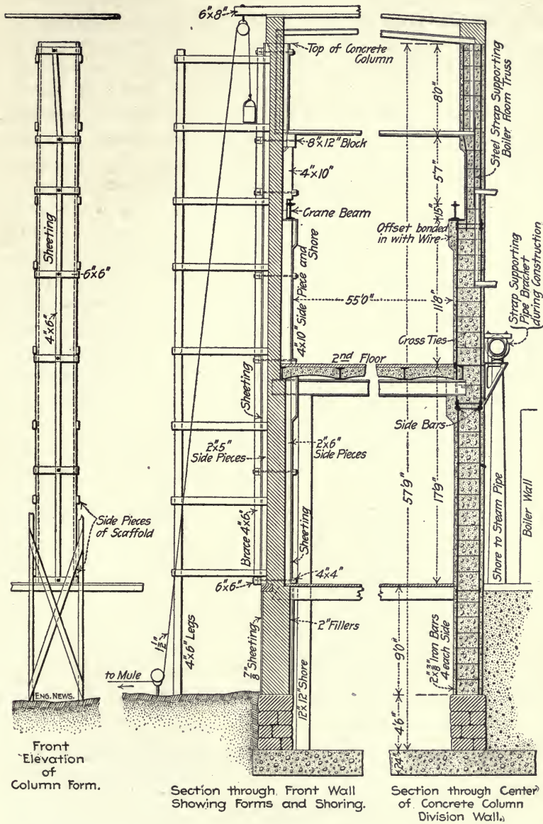
Fig. 224.—Staging and Forms Used in Building Column Shown by Fig. 223.
