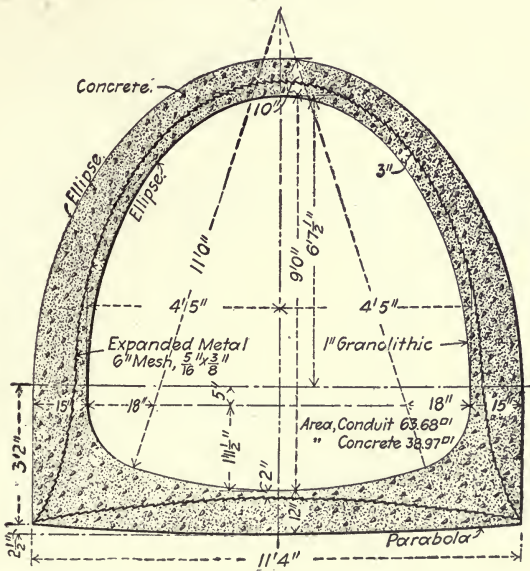
Fig. 253.—Section of 9-ft. Conduit, Philadelphia Filter Plant.
