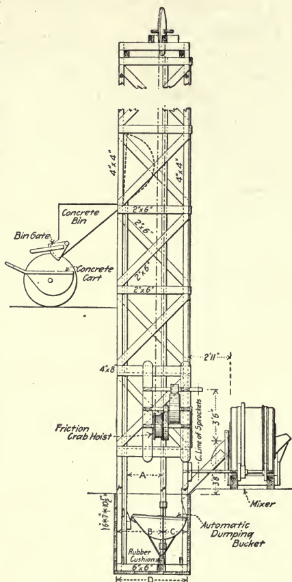
Fig. 218—Bucket Hoist for Building Work (Ransome).
