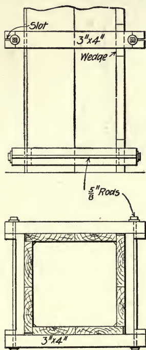
Fig. 178.—Form for Rectangular Column for Warehouse at St. Paul, Minn. with 2-in. lagging the form shown by Fig. 238 requires about 14 ft. B. M. of lumber per foot length of 12-in. column.
