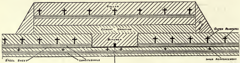
Fig. 270.—Bordenave Pipe for Swansea, England, Water Works.
