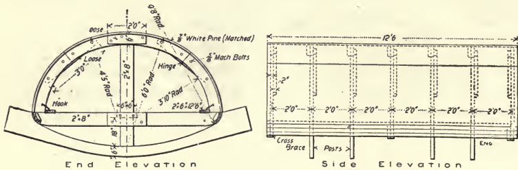
Fig. 173.—Center for Culvert at Kalamazoo, Mich.
