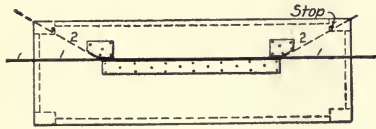
Fig. 208.—Table for Bending Reinforcing Bars.
