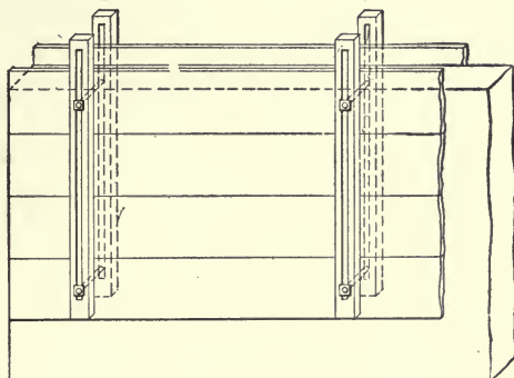
Fig. 204.—Movable Panel Form for Wall Construction.
