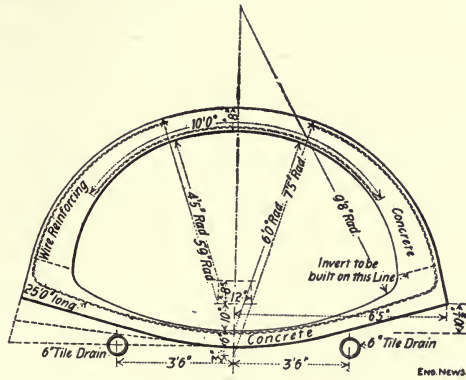
Fig. 172.—Cross-Section of Culvert at Kalamazoo, Mich.
