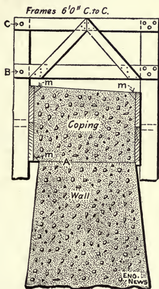
Fig. 103.—Sectional Form for Constructing Coping.
