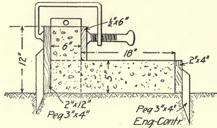
Fig. 123.—Continuous Form for Concrete Curb.
