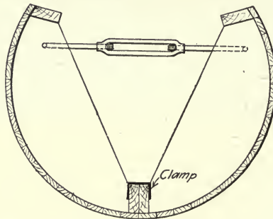
Fig. 249.—Invert Form for Conduit Construction.
