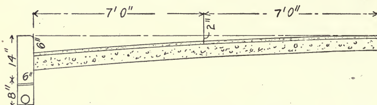
Fig. 119.—Concrete Pavement, Windsor, Canada.
