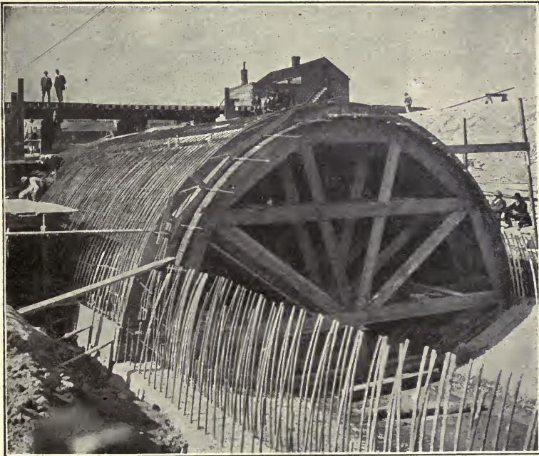
Fig. 262.—Center for Harlem Creek Sewer.
