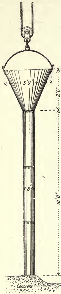
Fig. 33.—Steel Tremie for Depositing Concrete Under Water.
