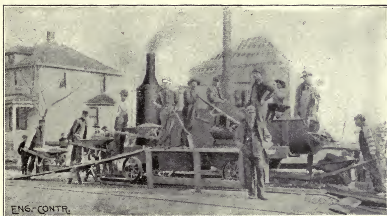
Fig. 112.—Foote Continuous Mixer Arranged for Pavement Foundation Work.
