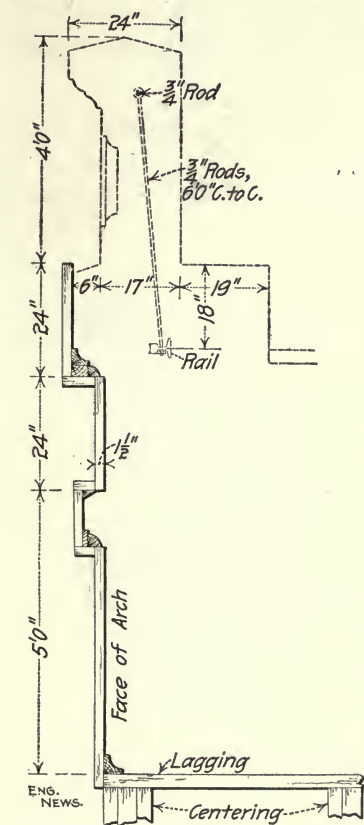
Fig. 293.—Spandrel Wall Mold for Arch Bridge.
