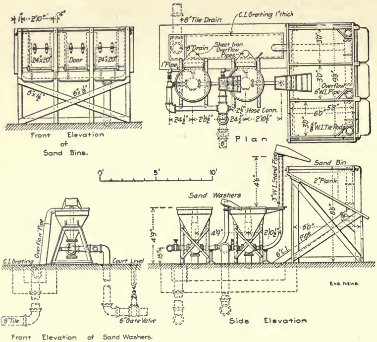
Fig. 1.—Plan and Elevation of Two-Hopper Ejector Sand Washing Plant. while the sand settles and is again ejected into a third hopper or to the stock pile or bins. The system may consist of
