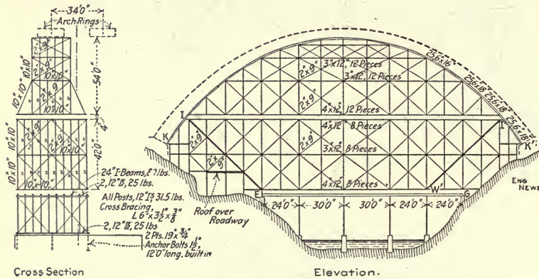
Fig. 151.—Center for 232-ft. Span Arch at Philadelphia, Pa.
