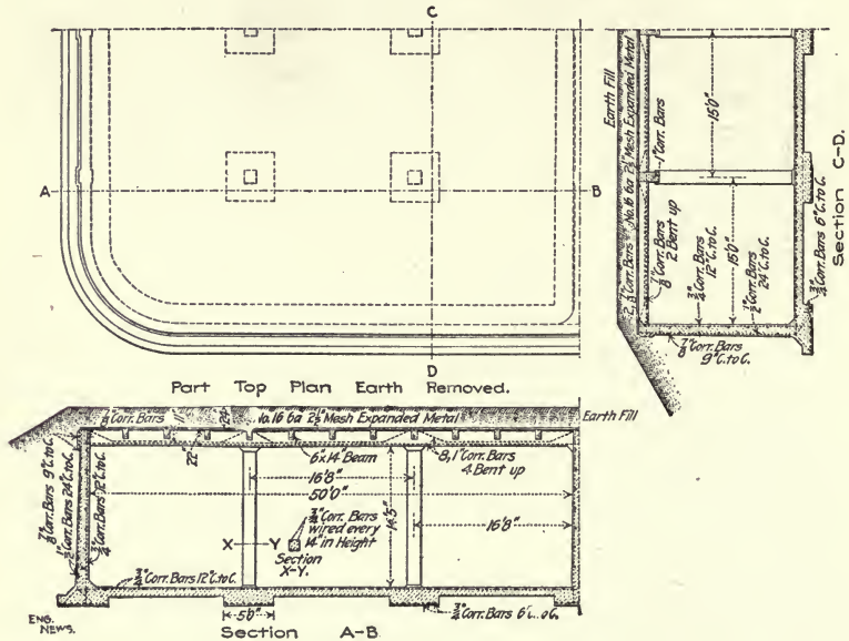
Fig. 277.—Reservoir at Ft. Meade, S. D.
