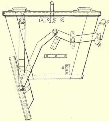
Fig. 30.—Stuebner Bucket for Depositing Concrete Under Water (Open Position).
