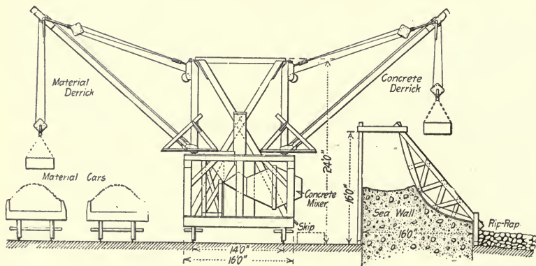
Fig. 107.—End Elevation of Traveling Mixer, Galveston Sea Wall.
