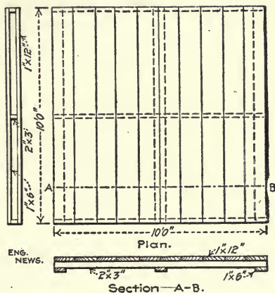
Fig. 44.—Portable Wooden Panels for Covering Floors.
