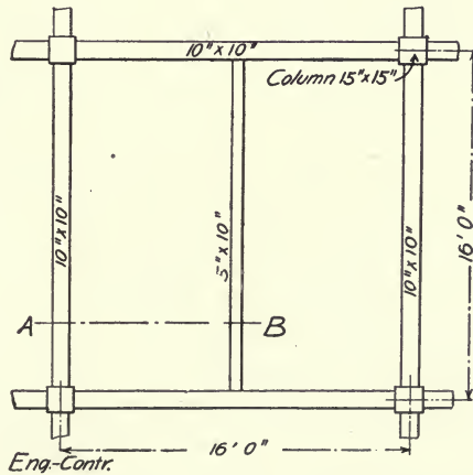
Fig. 225.—Girder Plan for 6-Story Building.
