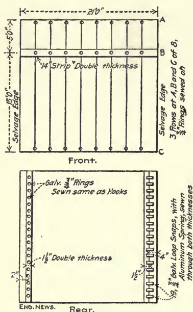
Fig. 42.—Canvas Curtain for Enclosing Open Walls.
