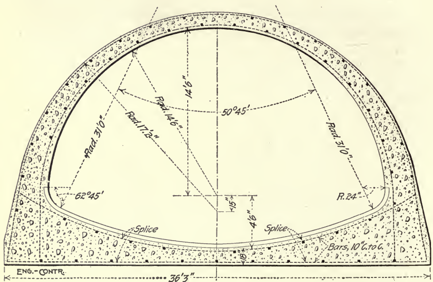
Fig. 261.—Harlem Creek Sewer, St. Louis, Mo.
