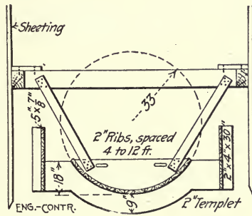
Fig. 257.—Form for South Bend Sewer (First Stage).
