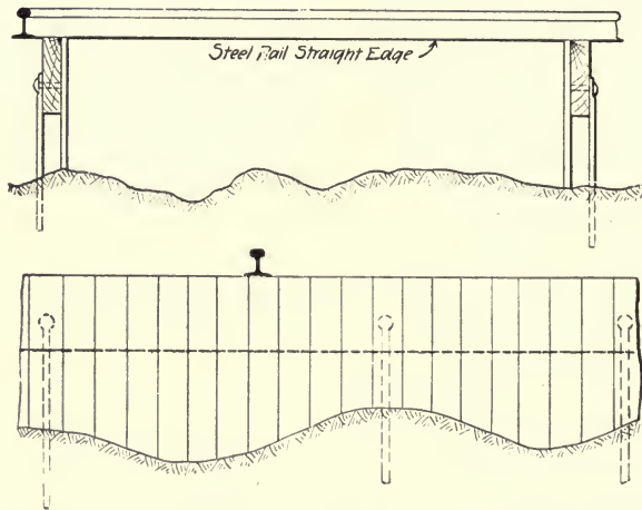
Fig. 32.—Form for Molding Footing for Block Concrete Breakwater.
