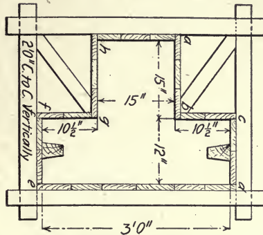
Fig. 181.—Form for T-Section Wall Column.
