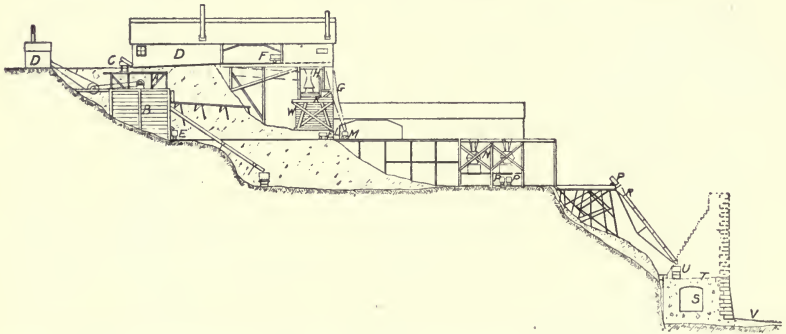
Fig. 70.—Concrete Making Plant for Constructing Lock Walls, Cascades Canal.
