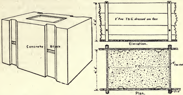
Fig. 81.—Concrete Blocks for Pier at Port Colborne Harbor.
