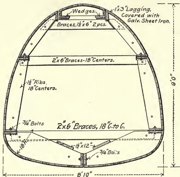
Fig. 254.—Form for 9-ft. Conduit Philadelphia Filter Plant.
