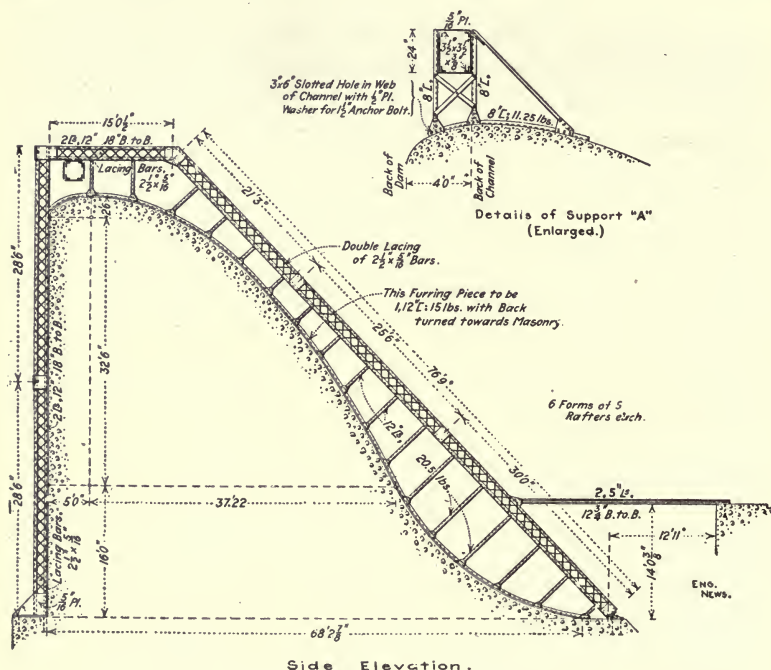
Fig. 90.—Steel Forms for McCall Ferry Dam.
