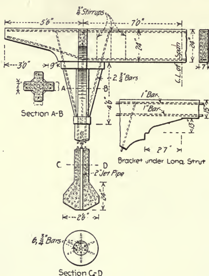
Fig. 60.—Concrete Pile for Pier at Atlantic City, N. J.
