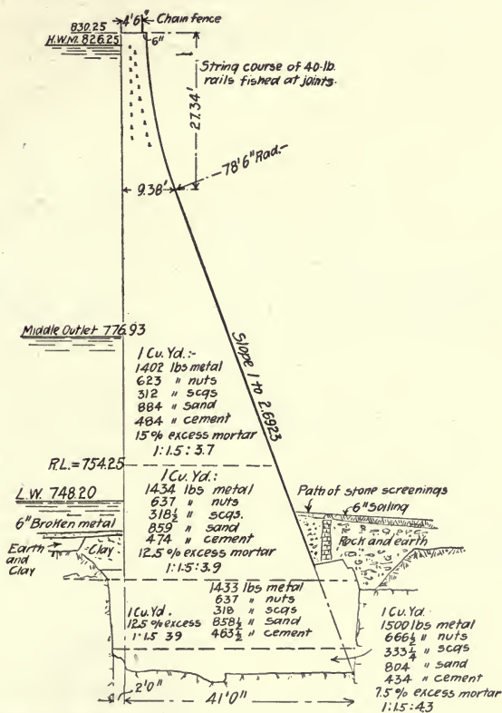
Fig. 36.—Cross-Section of Barossa Dam of Rubble Concrete.
