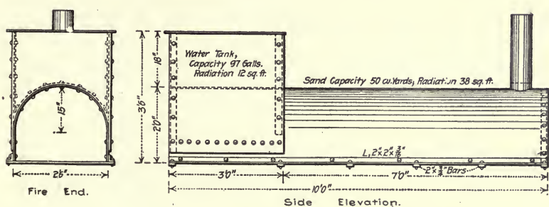
Fig. 40.—Portable Sand, Stone and Water Heater.
