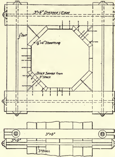
Fig. 187.—Form for Octagonal Column for Factory Building.
