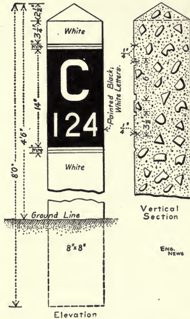
Fig. 306.—Mile Post, Chicago & Eastern Illinois Ry.
