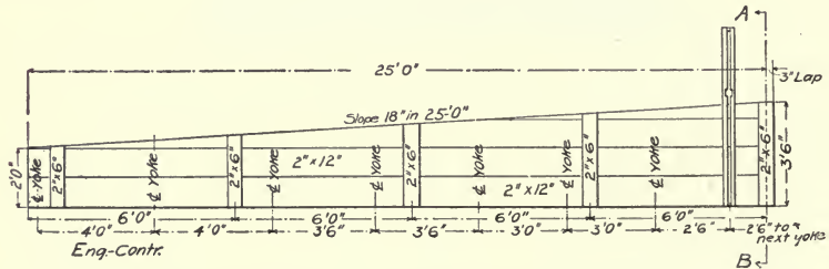
Fig. 242.—Forms for 50-ft. Roof Girders.
