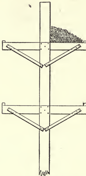
Fig. 207.—Rack for Storing Reinforcing Bars.
