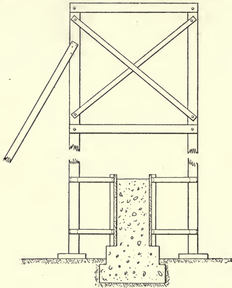
Fig. 201.—Continucus Form for Wall Construction.
