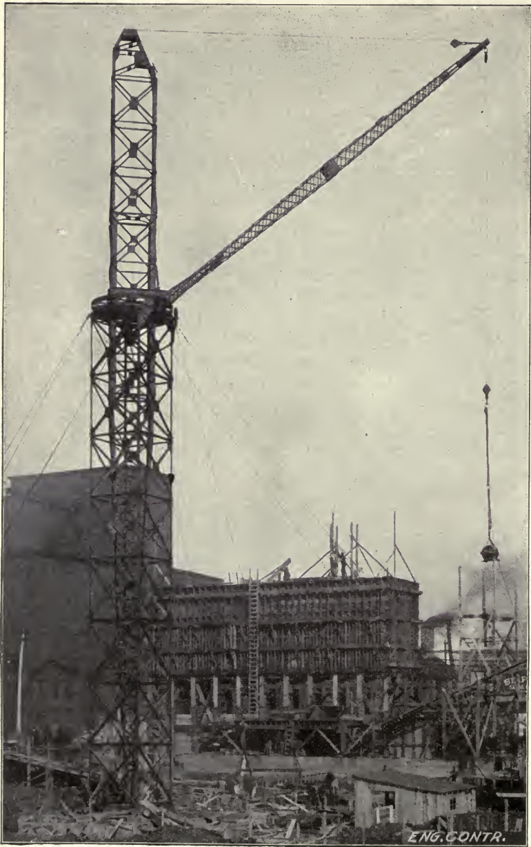
Fig. 221.—Derrick for Handling Concrete for Large Warehouse Building.
