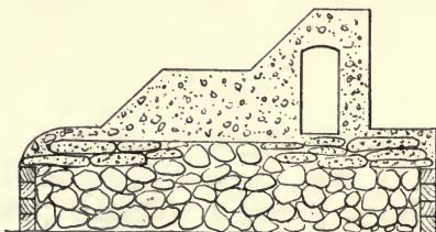
Fig. 78.—Cross Section of Marquette Breakwater Showing Manner of Constructing Footing with Bags of Concrete.
