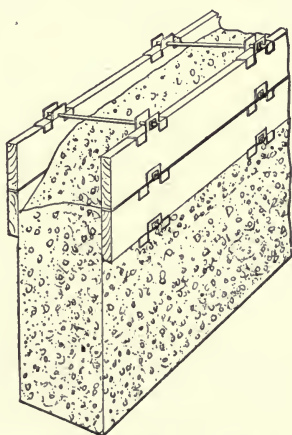
Fig. 205.—Sullivan's Plank Holders for Wall Forms.
