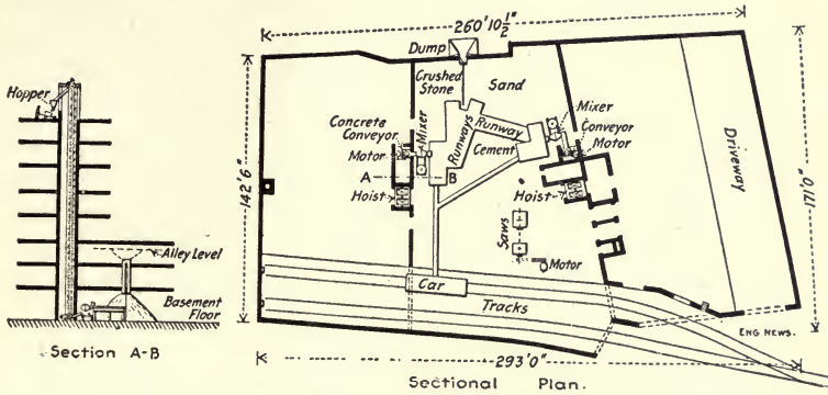
Fig. 219.—Plan of Concrete Mixing and Handling Plant for 9-Story Building.
