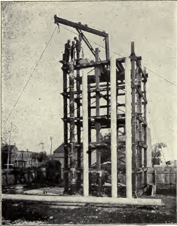
Fig. 59.—Plant for Vertical Molding of Concrete Piles.
