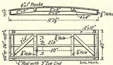
Fig. 282.—Form Panels for Circular Reservoir Wall.
