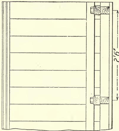
Fig. 183.—Core Form for Hollow Column.
