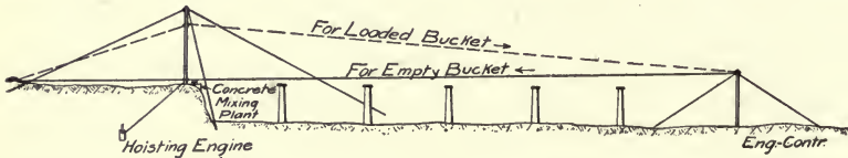
Fig. 151a.—Cableway for Concreting Bridge Piers.
