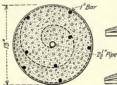
Fig. 65.—Cross-Section of Chenoweth Rolled Pile.
