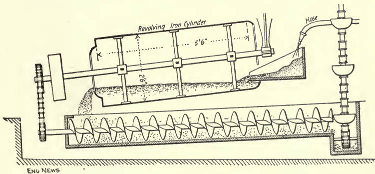
Fig. 6.—Details of Rotating Tank Sand Washer Used at Hudson, N. Y.
