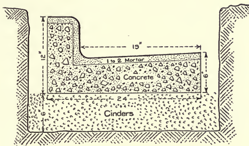
Fig. 125.—Concrete Curb and Gutter at Champaign, Ill.
