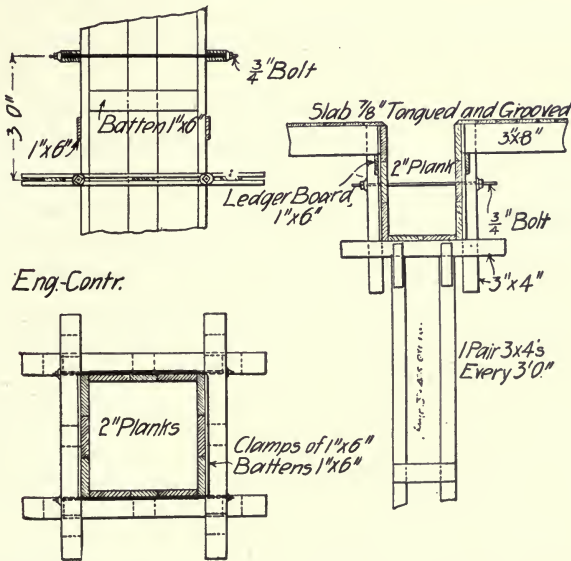
Fig. 238.—Column and Floor Forms for Four-Story Garage.
