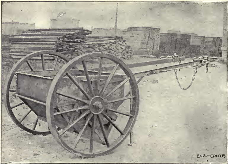
Fig 113.—Briggs Cart Distributing Concrete for Pavement Foundation.
