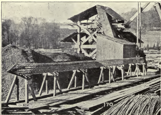
Fig. 63.—View Showing Method of Fabricating Reinforcement for a Round Pile with Flattened Sides.
