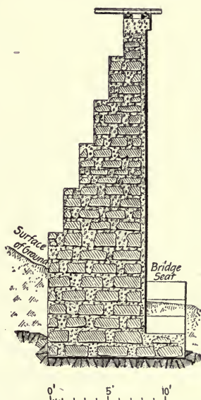
Fig. 38.—Bridge Abutment of Rubble Concrete.
