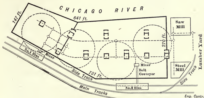
Fig. 220.—Plan of Concrete Mixing and Handling Plant for Large Warehouse Building.
