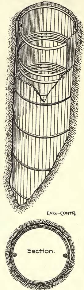
Fig. 53.—Curbing for Concrete Piers (Usual Construction).
