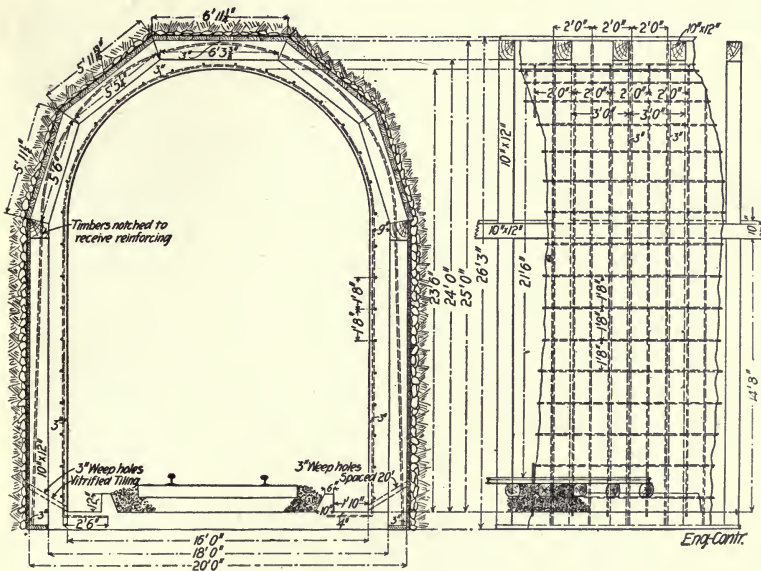
Fig. 138.—Sections Showing Concrete Lining for Burton Tunnel.
