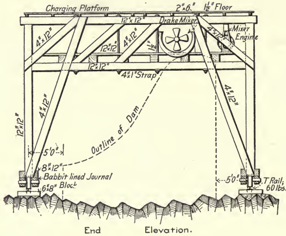
Fig. 92.—Traveler for Concreting Dam, Chaudiere Falls, Quebec.
