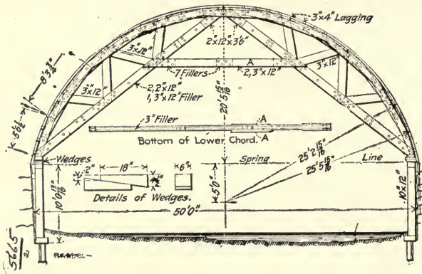
Fig. 149.—Center for 50-ft. Arch Span (Cocket).
