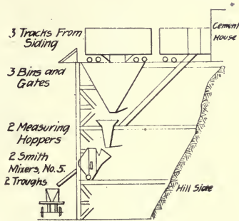
Fig. 15.—Side Hill Mixing Plant.
