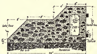
Fig. 77.—Cross Section of Marquette Breakwater.
