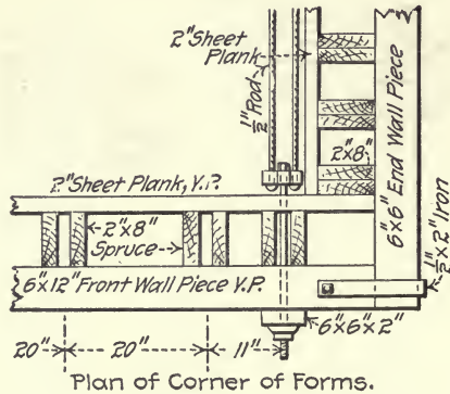
Fig. 111.—Corner Detail of Retaining Wall Forms, New York Central Terminal Work.
