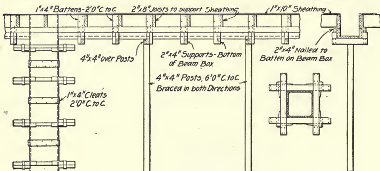
Fig. 197.—Girder and Slab Form for Concrete Building Work.
