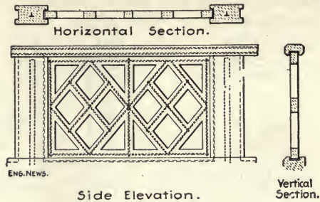
Fig. 290.—Railing for Arch Bridge.
