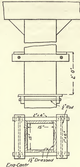
Fig. 226.—Column Form for 6-Story Building.
