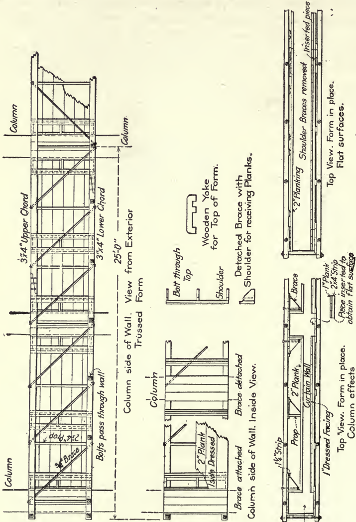
Fig. 235.—Details of Wall Form Panel for One-Story Building.
