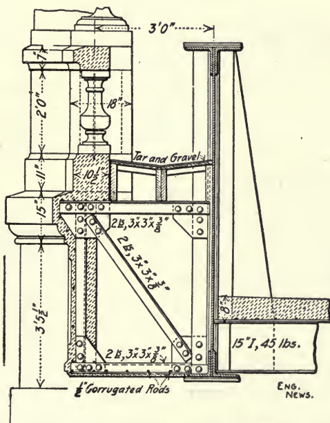
Fig. 298.—Concrete Facade for Plate Girder Bridge.
