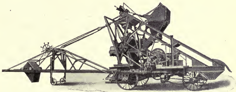
Fig. 115.—Chicago Improved Cube Traction Mixer for Pavement Foundation.
