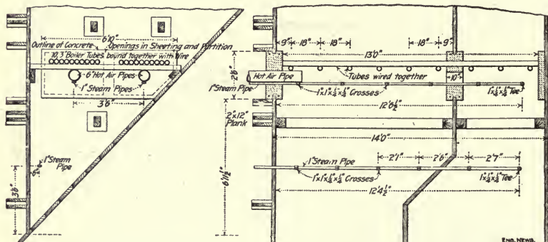
Fig. 41.—Bin Arrangement for Heating Sand and Stone.
