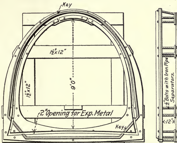
Fig. 255.—Bulkhead Form for Conduits, Philadelphia Filter Plant.
