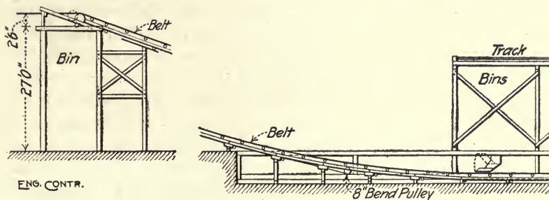
Fig. 13.—Belt Conveyor Transporting Sand and Gravel.
