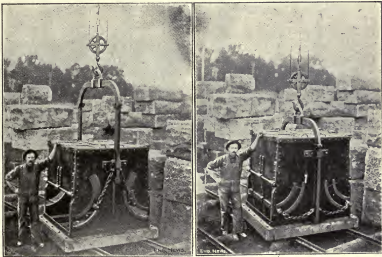
Fig. 26.—O'Rourke Bucket for Depositing Concrete Under Water.
