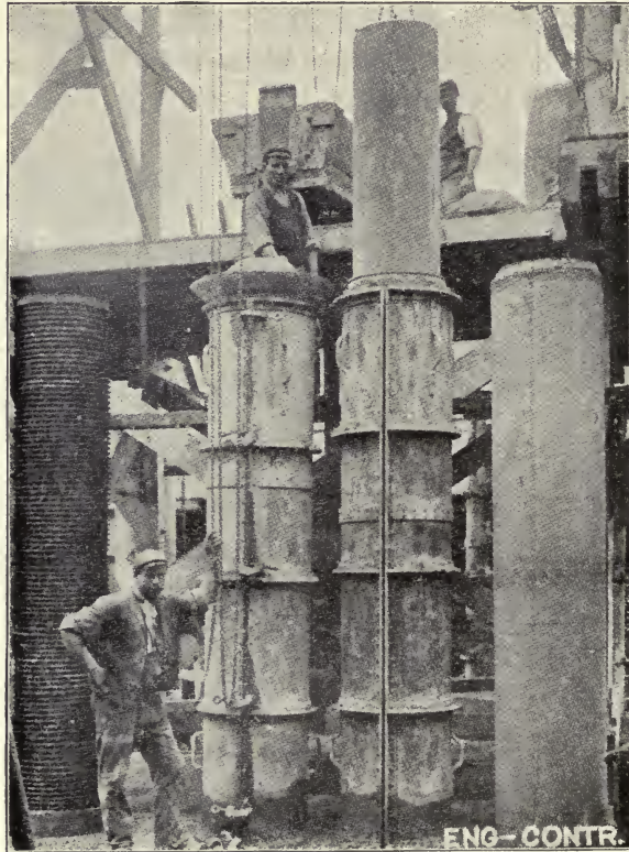
Fig. 272.—Casting Bordenave Pipe at Swansea, England.
