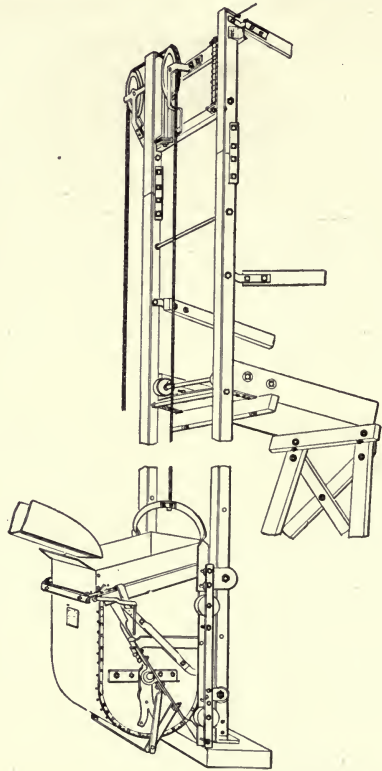
Fig. 214.—Bucket Hoist for Building Work (Wallace-Lindesmith).
