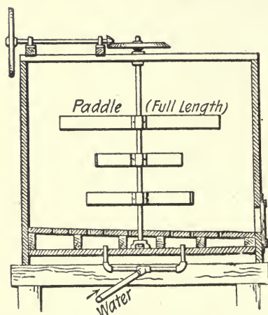
Fig. 4.—Details of Tank Washer Used at Springdale, Pa.
