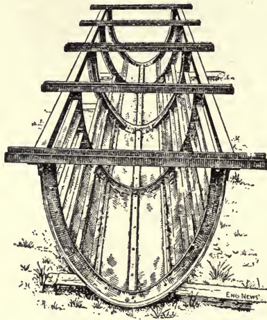
Fig. 263.—Invert Form for Sewer Construction.
