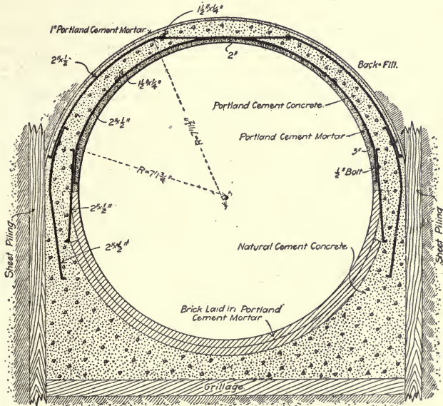
Fig. 264.—Sewer at Cleveland, Ohio.
