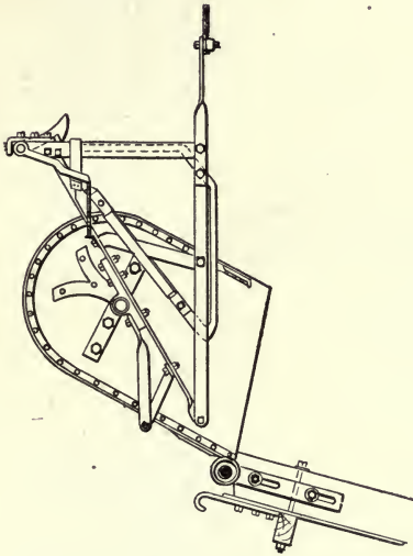
Fig. 215.—Wallace-Lindesmith Hoist Bucket in Discharging Position.
