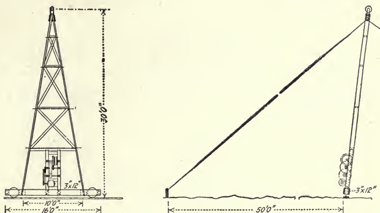
Fig. 232.—Derrick for Stripping Wall Column Forms Shown by Fig. 230.
