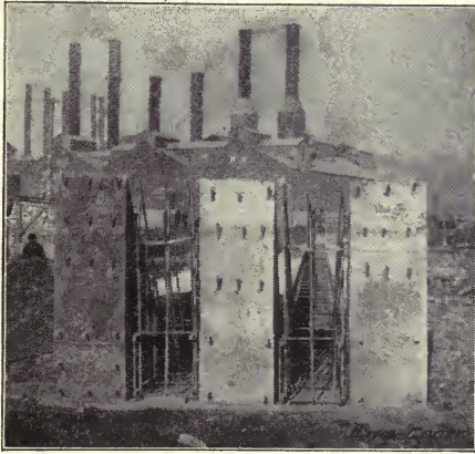
Fig. 240.—Arrangement for Molding Ten Single-Bracket Columns.
