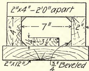
Fig. 292.—Form for Hand Rail Shown by Fig. 290.
