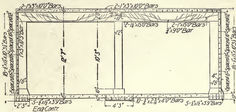
Fig. 275.—Transverse Section of 75,000-Gallon Reservoir.
