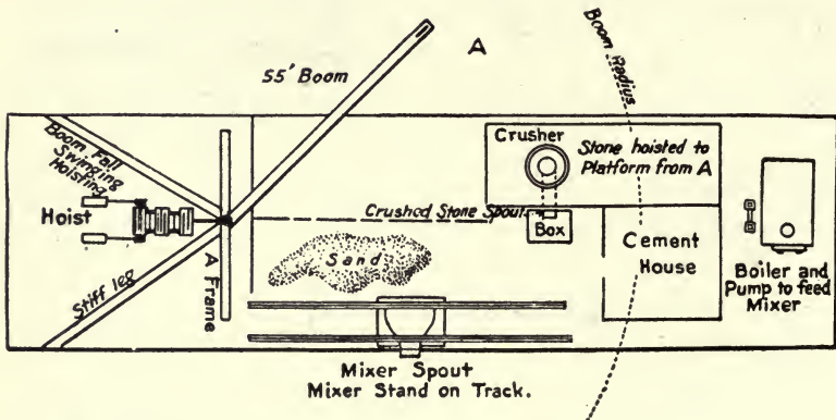
Fig. 84.—Scow Plant for Mixing and Placing Concrete, Port Colborne Harbor Pier.
