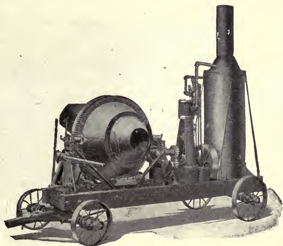
Fig. 21.—Smith Concrete Mixer.
