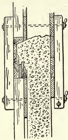
Fig. 295.—Example of Poor Wall Form Construction.
