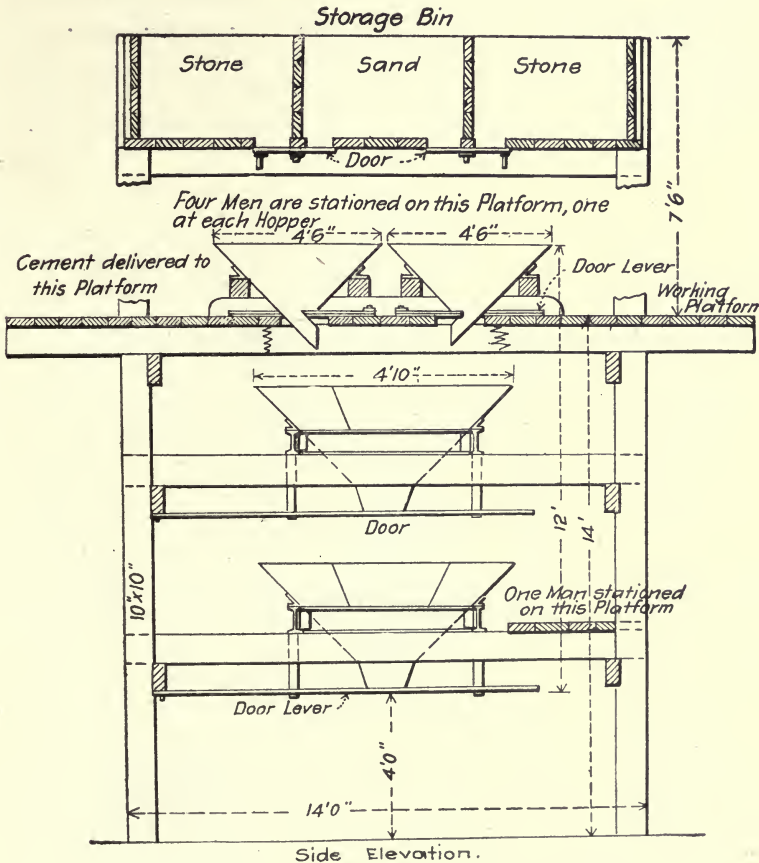
Fig. 24.—Hains Gravity Mixer, Fixed Hopper Form.
