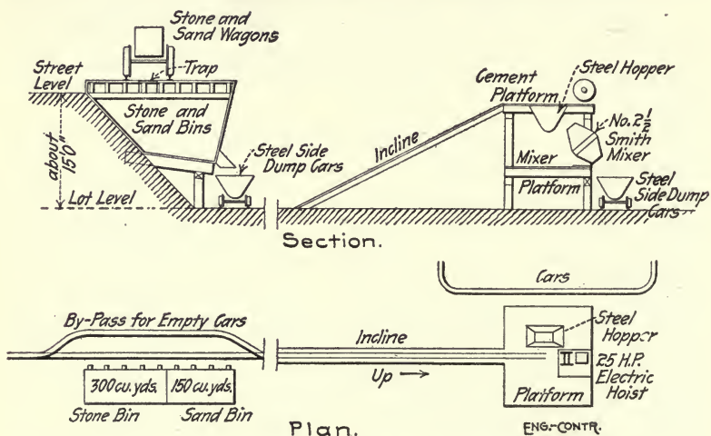
Fig. 58.—Arrangement of Concrete Making Plant, Concrete Pier Construction was maintained with a force of 25 men. In all some 17,000 cu. yds. of concrete were mixed and deposited.
