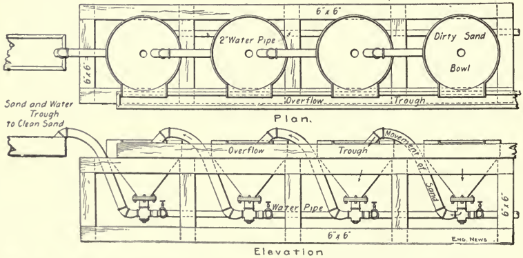
Fig. 2.—Plan and Elevation of Four-Hopper Ejector Sand Washing Plant. anywhere from two to six hoppers. Figure 1 shows a two-hopper lay-out and Fig. 2 shows a four-hopper lay-out. In
