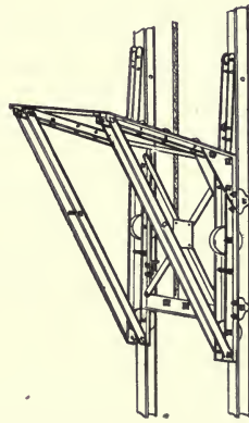
Fig. 216.—Lumber Carriage for Wallace-Lindesmith Hoist.
