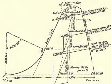
Fig. 35.—Diagram Cross-Section of Rubble Concrete Dam, Chattahoochee River.
