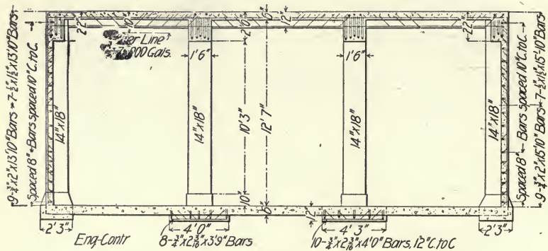
Fig. 274.—Longitudinal Section of 75,000-Gallon Reservoir.
