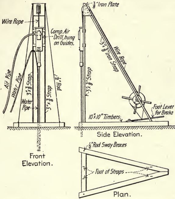
Fig. 303.—Device for Drilling Green Concrete.
