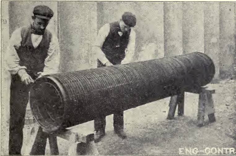
Fig. 271.—Applying External Reinforcement to Bordenave Pipe.
