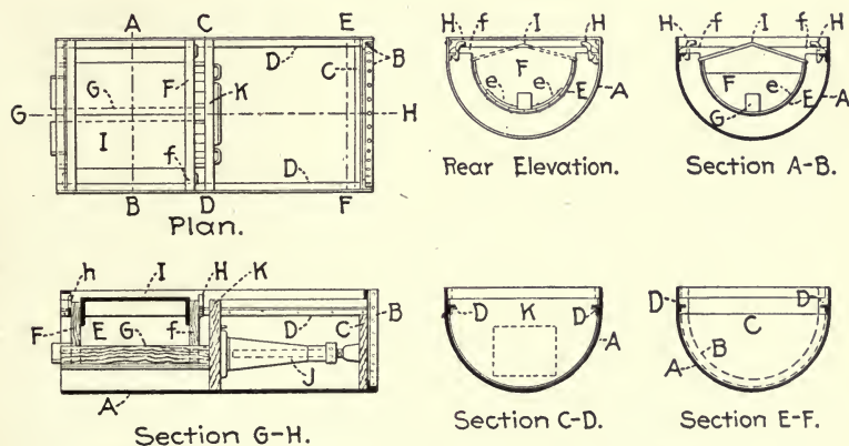
Fig. 260.—Traveling Invert Form for Sewer Construction.
