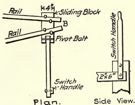
Fig. 164.—Improvised Switch for Service Cars, General Plan.
