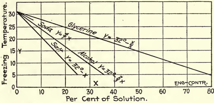
Fig. 39.—Diagram Showing Effect on Freezing Point of Water by Admixture of Various Substances.
