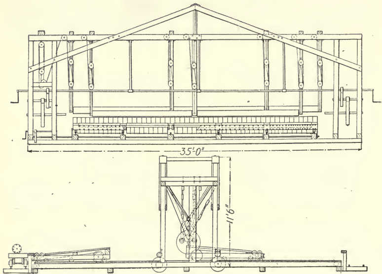
Fig. 67.—Machine for Rolling Chenoweth Piles.
