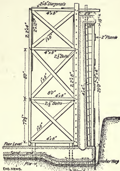
Fig. 281.—Frame for Forms for Circular Reservoir Wall.
