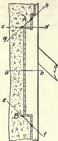
Fig. 294.—Diagram Illustrating Details of Mold Construction.
