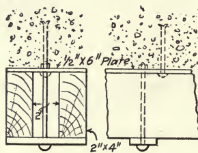
Fig. 283.—Sketch Showing Filler for Joint Between Form Panels.
