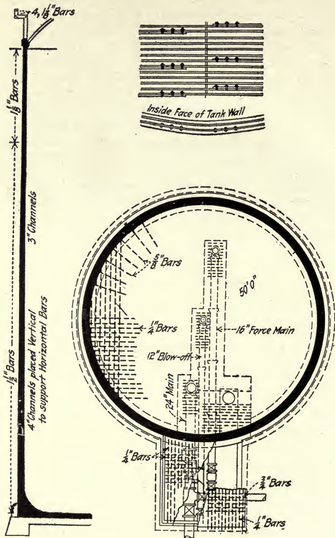
Fig. 279.—Standpipe at Haverhill, Mass.
