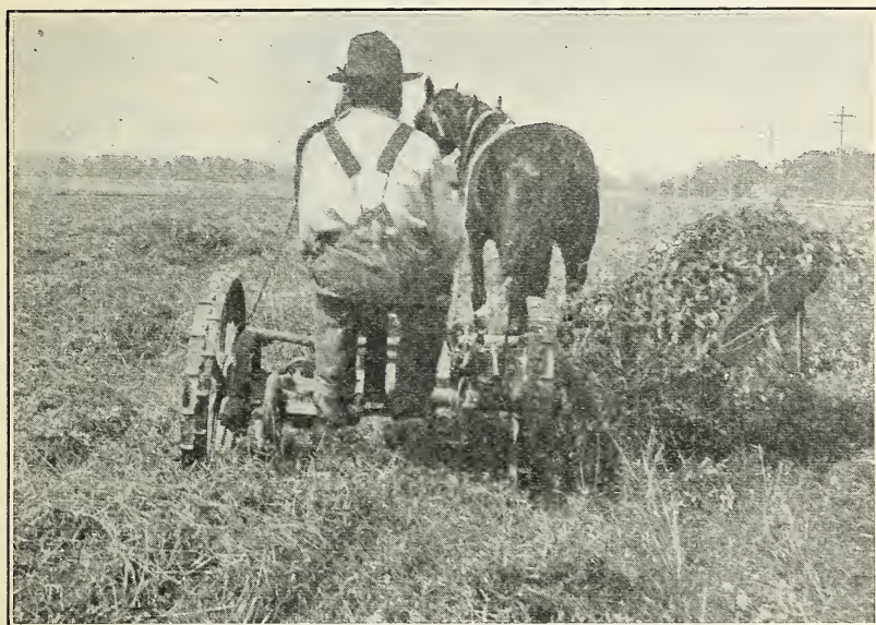
FIG. 4.—Harvesting semigreen hairy vetch with a mowing machine. Note the tangled mass that clings to the cutter bar. This difficulty can be largely overcome by the use of a swather attachment.
