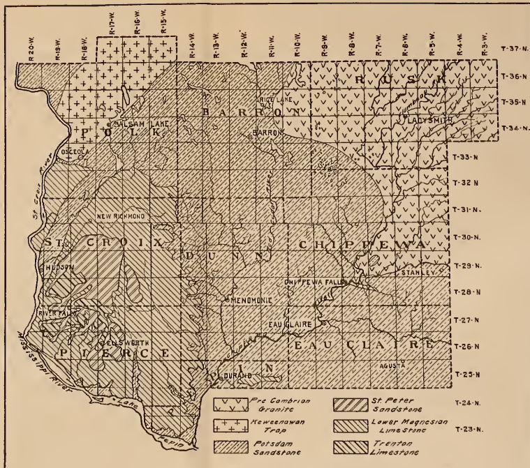
GEOLOGICAL MAP OF THE NORTHWESTERN AREA.
