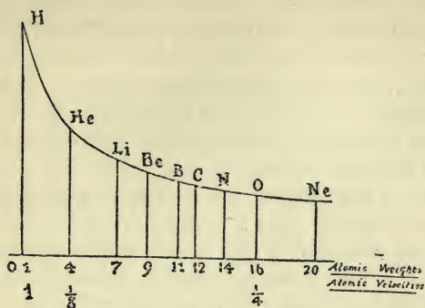
FIG. 9. Diagram of Atomic Velocity.
