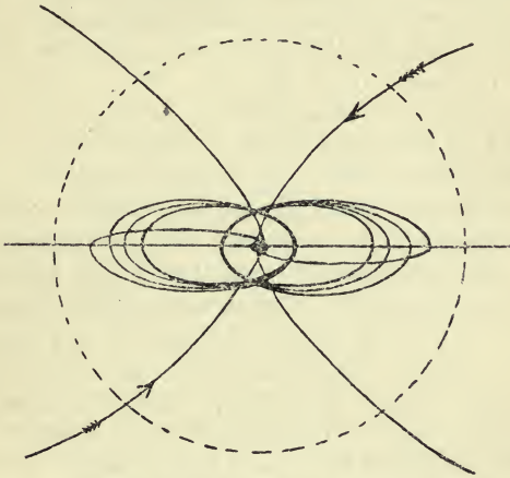
FIG. 13.—DIAGRAM SHOWING THE FORMATION OF THE ORBIT OF A DOUBLE STAR.
