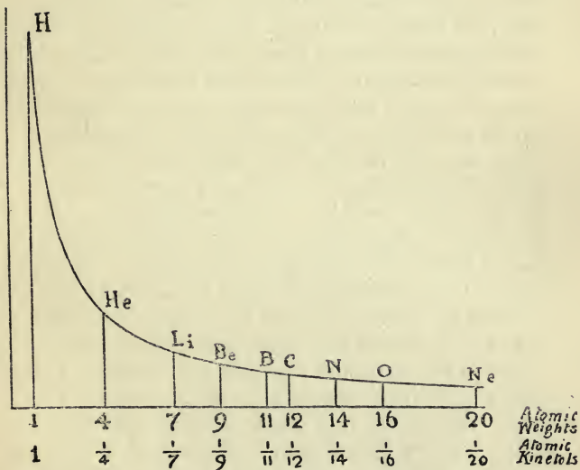
FIG. 10. Diagram of Atomic Kinetol.
