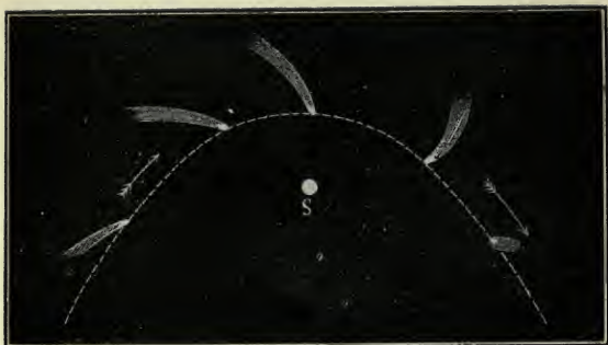
FIG. 12.—DIAGRAM OF COMET'S ORBIT. The above diagram illustrates also the direction of the tail.
