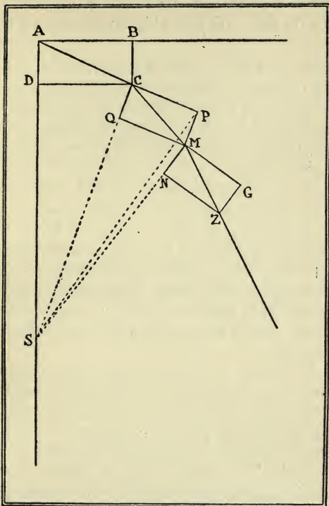
FIG 15.—DIAGRAM OF THE ORBIT OF A PLANET.
