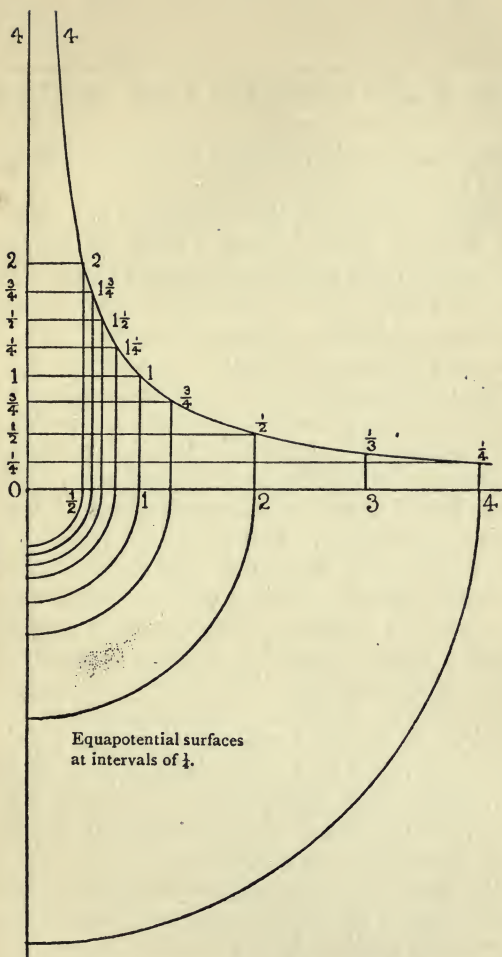
FIG. 6.—The Kinetic Curve. An Equilateral Hyperbola. Curve of Potential of Kinetol or of Thermatol.
