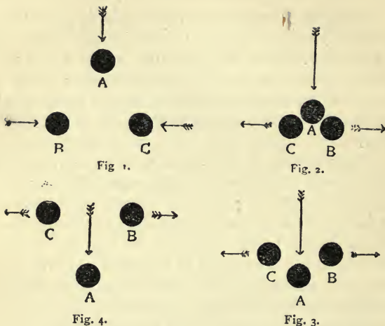
FIG. 14.—DIAGRAM ILLUSTRATING CHANGES OF VELOCITY THAT MAY OCCUR WHEN THREE STARS PASS NEAR ONE ANOTHER.
