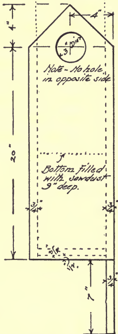
SIDE ELEVATION
