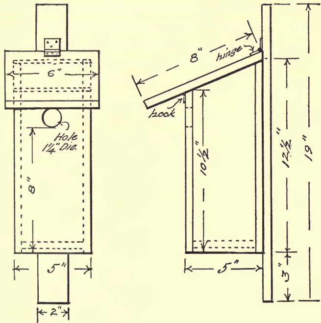
FRONT ELEVATION
