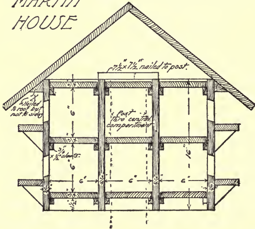
Plans for a Martin house—Elevations
