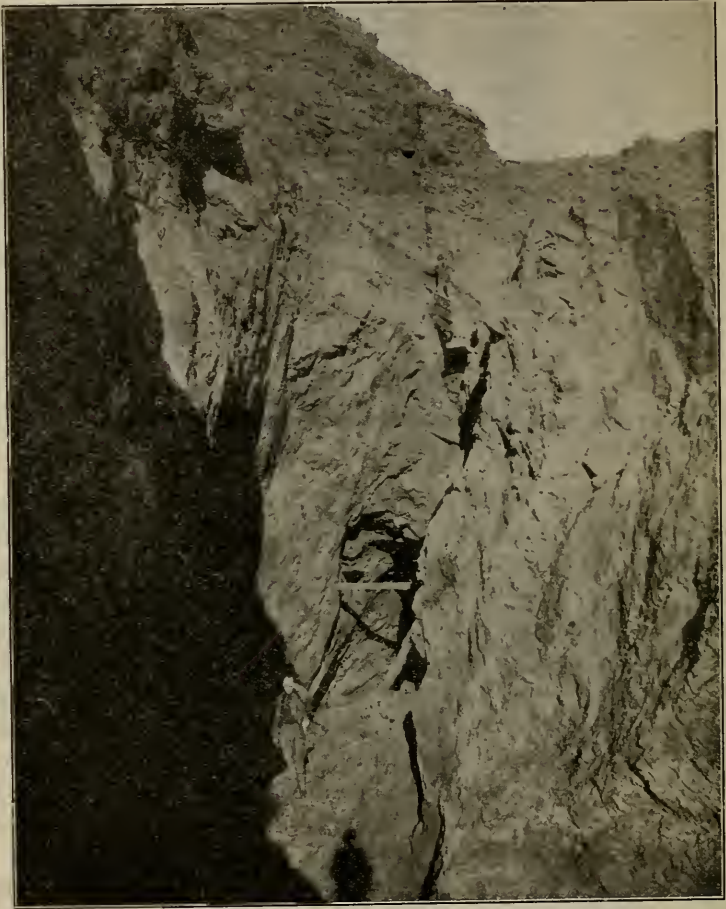
Open-cut stope of Buckeye Manganese Mine, Stanislaus County. Ore body extracted was 20' wide and over 75' long, of ore carrying 48% manganese. This mine was the largest single producer in California in 1918-1919.
