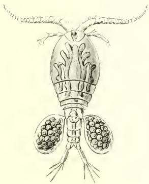
Fig. 2 — Cyclope commun.
