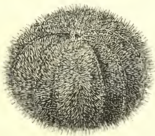
Fig. 272. — Oursin comestible.
