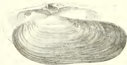
Fig. 4 — Lutraria elliptica
