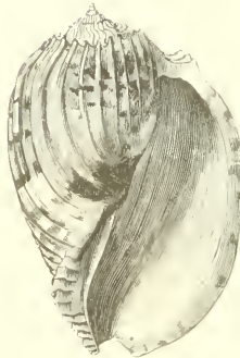
Fig. 5 — Harpe noble
