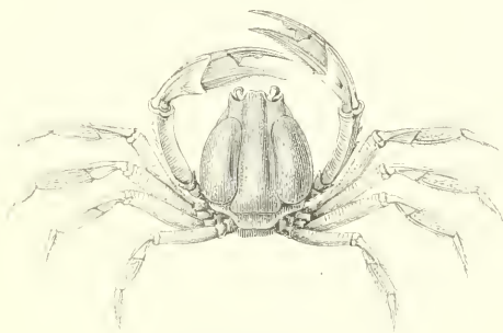
Fig. 15 — Mictyre longicaepe.
