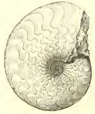
Fig. 106. — Goniatite semipartic.
