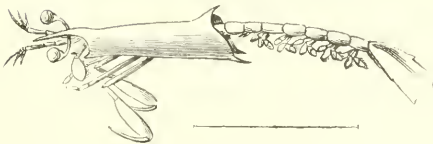
Fig. 2. — Aline hydric.
