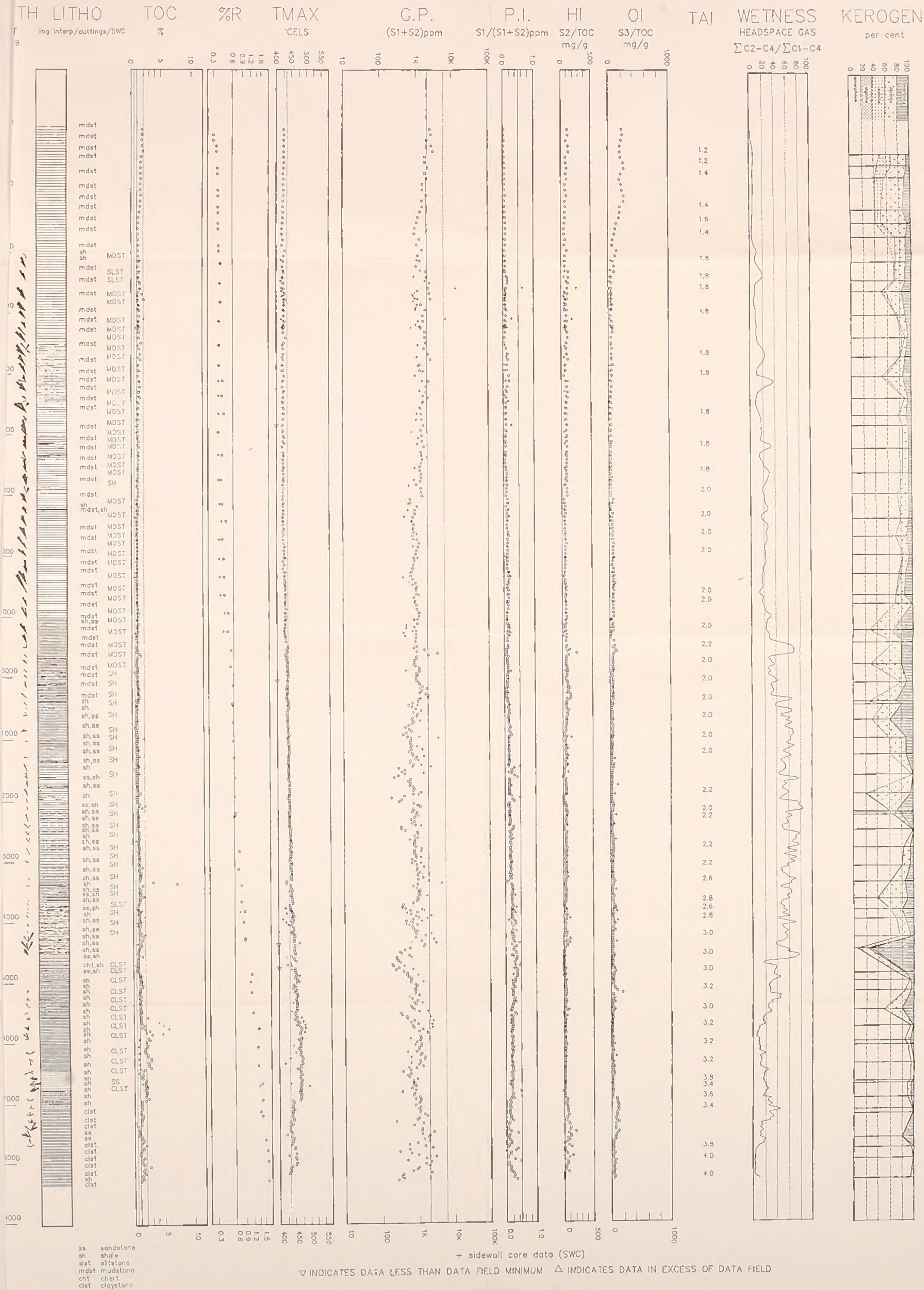
PLATE 3. GEOCHEMICAL DATA
