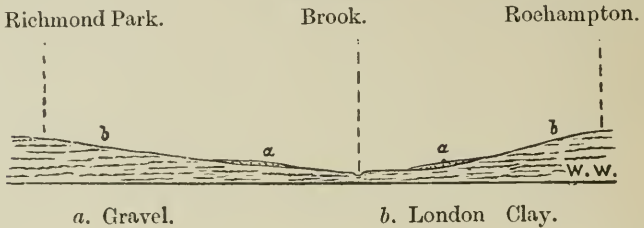
Fig. 16.—Section from Richmond Park to Roehampton (W. Whitaker.) *
