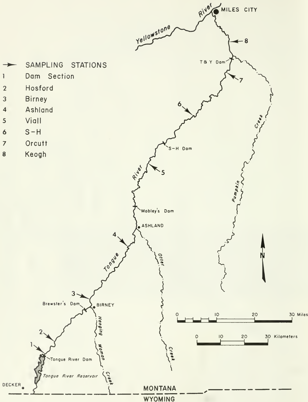
Figure 3. Tongue River sampling stations.
