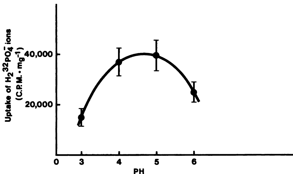
Figure 1. Relationship between pH and uptake of H_2^{32}PO_4 ions by brown ectomycorrhizae of Abies balsamea .
