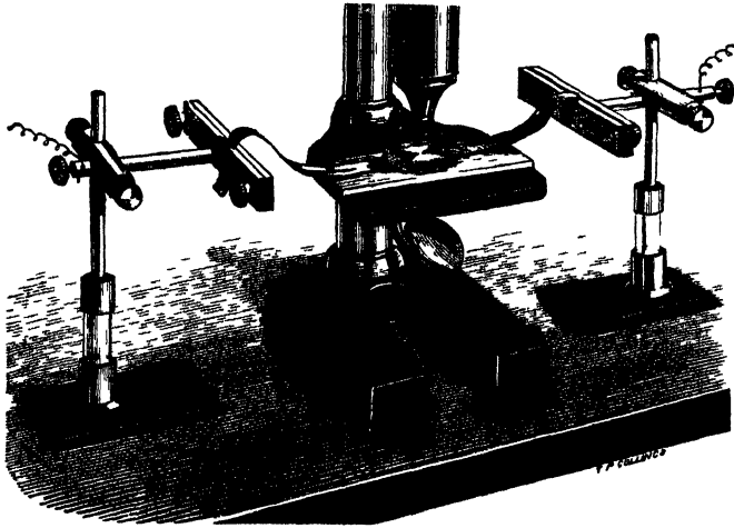
FIG. 42 — APPARATUS ARRANG'D FOR TRANSMITTING ELECTRICITY.
