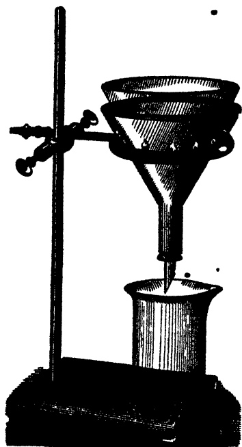
FIG. 4. HOT-WATER FILTERING APPARATUS WITH RING BURNER.
