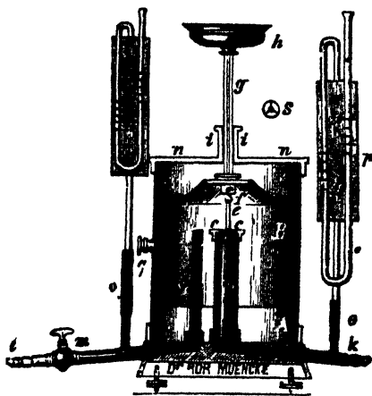
FIG 19 MOITESSIER'S GAS-PRESSURE REGULATOR
