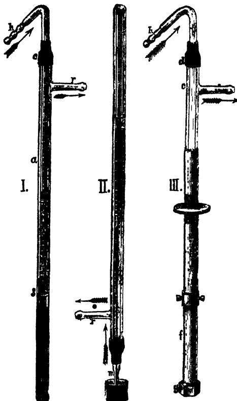
FIG. 23.—MEYER'S THERMO-REGULATOR.
