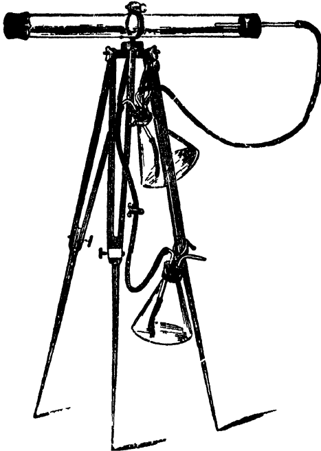
FIG 44.—HESSE'S APPARATUS
