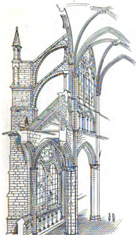
SECTION AND DETAIL OF CATHEDRAL AT AMIENS
