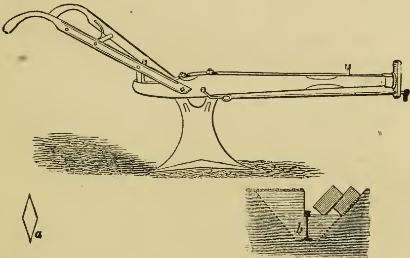
FIG. 6.—Wrought Iron and Steel Sub-soil Plow.
