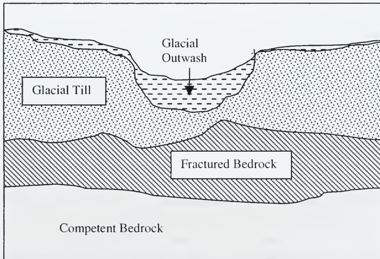
FIGURE 5 OUTWASH VALLEY CROSS SECTION
