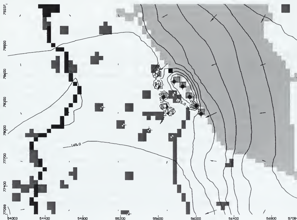
FIGURE 18 MODFLOW RESULTS. PUMPING RATE - 4 GPM
