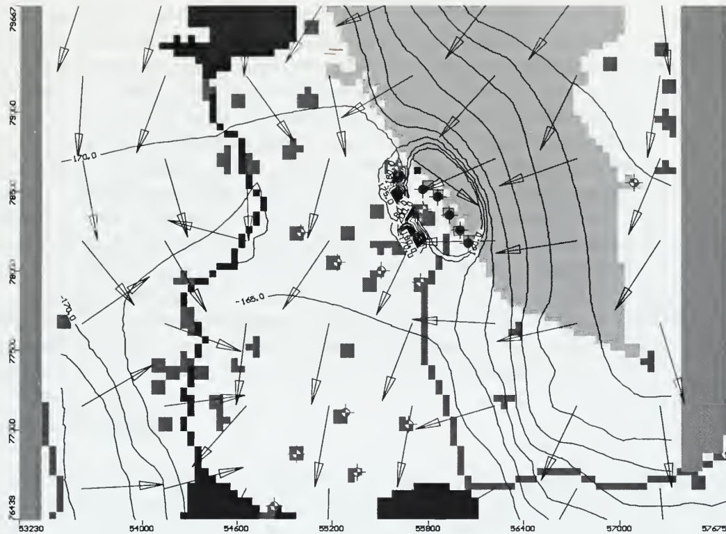
FIGURE 22 MODFLOW RESULTS. PUMPING RATE - 20 GPM
