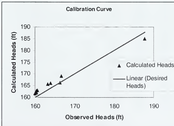
FIGURE 9 CALIBRATION CURVE
