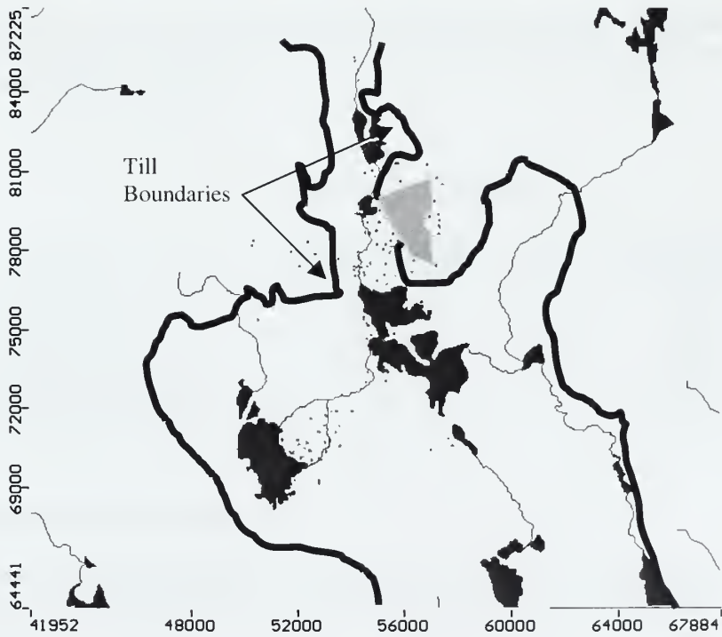
FIGURE 8 TILL BOUNDARIES
