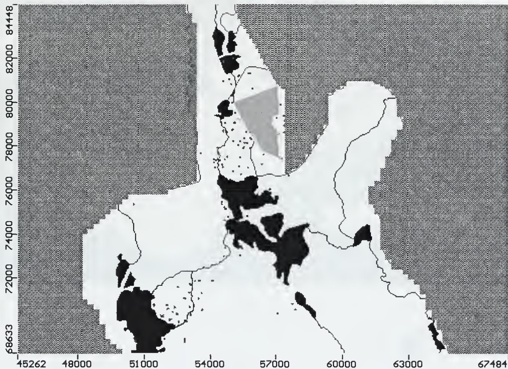
FIGURE 6 MODEL AREA
