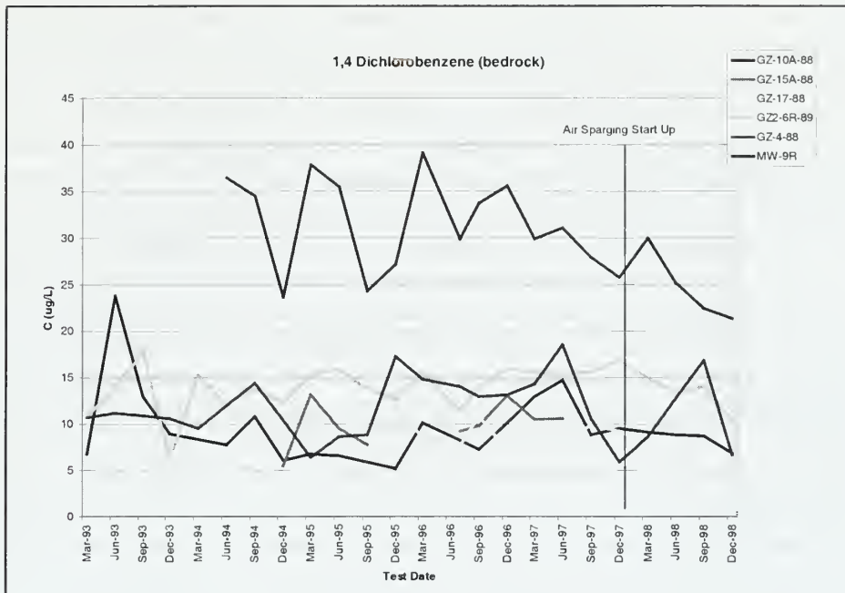
FIGURE 14 1,4-DICHLOROBENZENE CONCENTRATIONS IN THE BEDROCK
