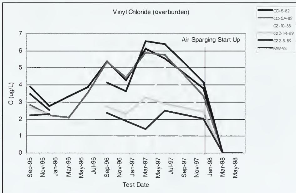
FIGURE 11 VINYL CHLORIDE CONCENTRATIONS IN THE OVERBURDEN ZONE
