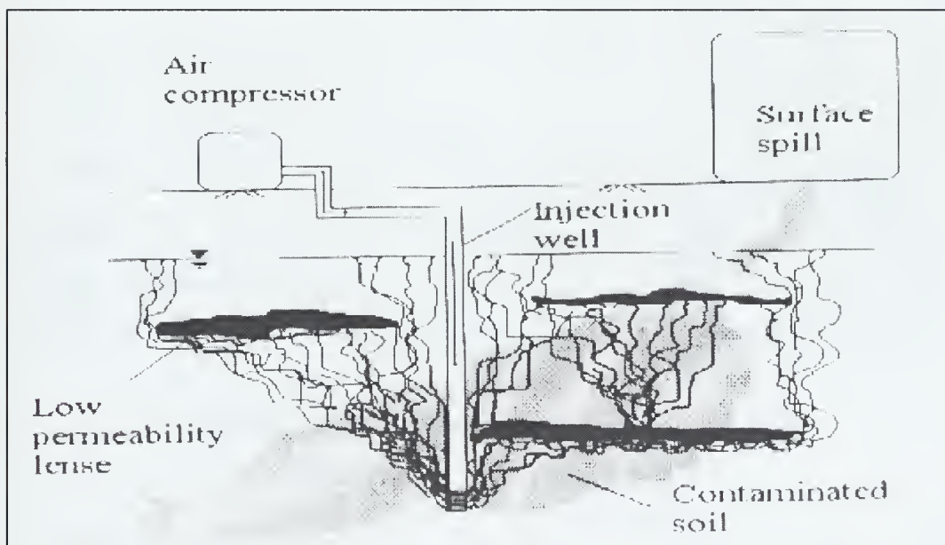
FIGURE 15 SCHEMATIC OF AIR SPARGING SYSTEM (MARULANDA, 1998)
