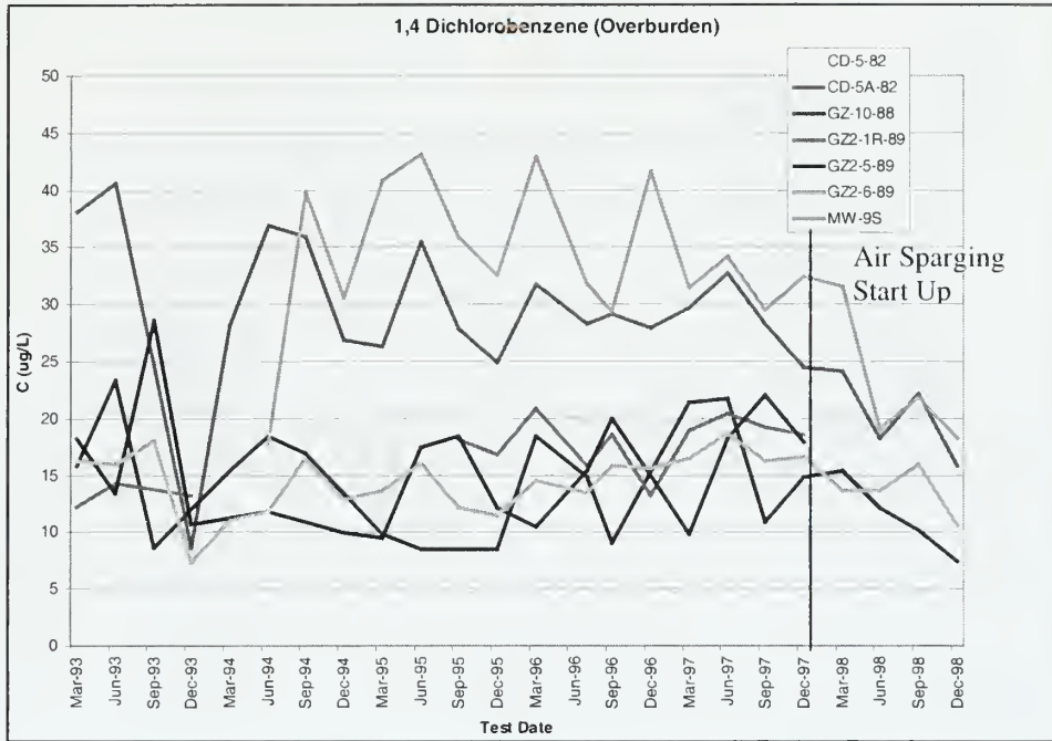
FIGURE 12 1,4-DICHLOROBENZENE CONCENTRATIONS IN THE OVERBURDEN ZONE
