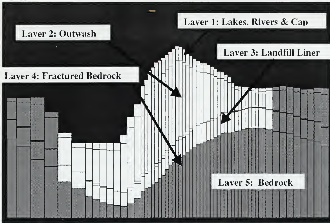
FIGURE 7 MODEL LAYERS
