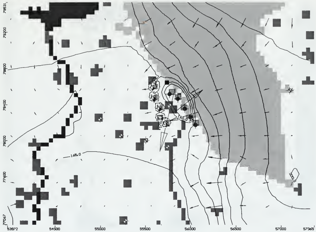
FIGURE 20 MODFLOW RESULTS. PUMPING RATE – 5 GPM
