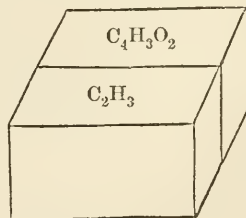
Acetone.
