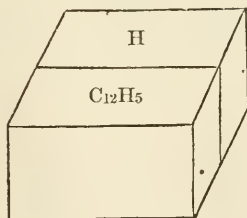
Benzole.
