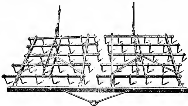
FIG. 80. Spike-tooth harrow.
