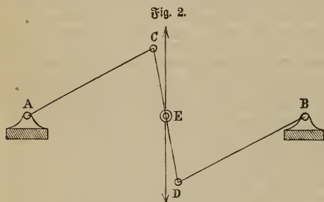
Watts Lemniskoidenlenker.
