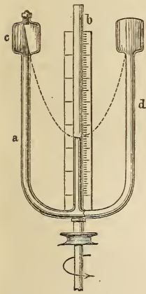
Brown's Gyrometer.
