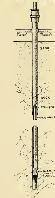
HOW A PLUNGER-ELEVATOR IS BUILT.
