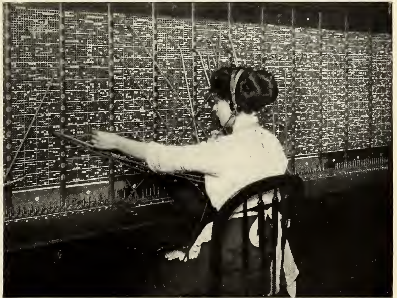
AN OPERATOR AT THE "B" BOARD. WITHIN HER REACH ARE TEN THOUSAND AND TWO HUNDRED "JACKS."
