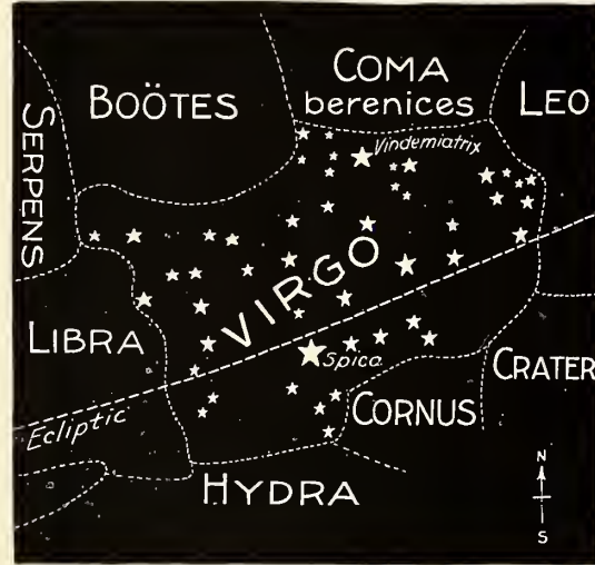
A MAP OF VIRGO AND SURROUNDING CONSTELLATIONS.
