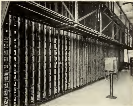
THE DISTRIBUTING FRAME WHERE THE WIRES ARE CONNECTED TO A PERFECT MAZE OF SAFETY DEVICES.
