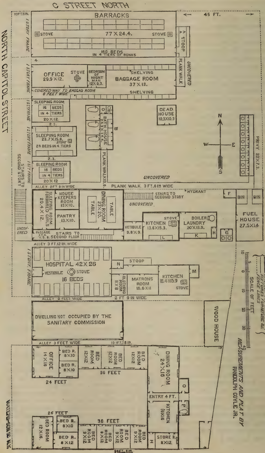
GROUND PLAN OF THE "HOME" AT WASHINGTON, D. C.
