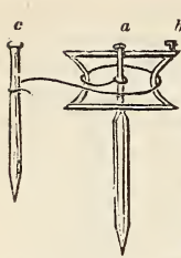
Fig. 101. Iron reel and pin for a garden-line.
