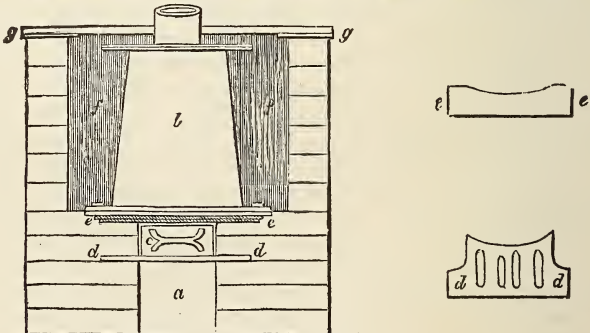
Fig. 148. Mode of setting Rogers's conical boiler.
