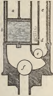
Fig. 82. Section of Read's pneumatic hand-engine.
