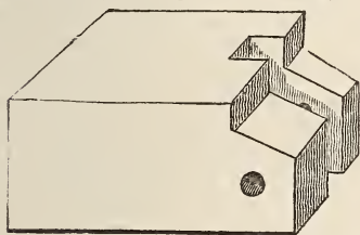
Fig. 116. Stone for fixing temporary rafters.
