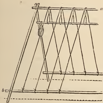
Fig. 378. Prop for Climbing Plants.
