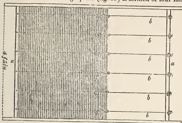
Fig. 89. Mode of making straw mats.
