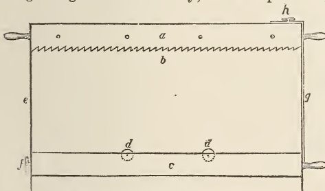
Fig. 261. Side view of the girdling machine.
