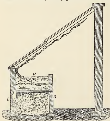
Fig. 136. Section of a vinery heated by dung.
