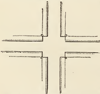
Fig. 126. Plan showing the intersection of trellised walks.
