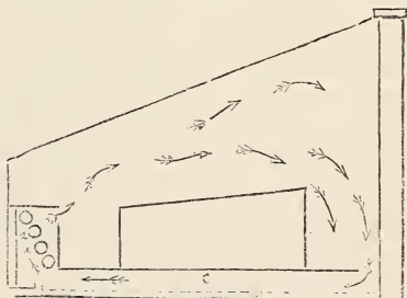
Fig. 2. Section of a Hothouse heated by hot water according to Mr. Penn's manner.
