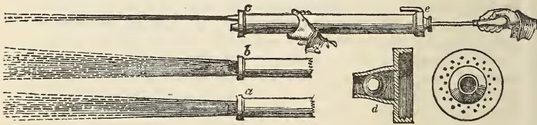
Fig. 80. Read's garden syringe.
