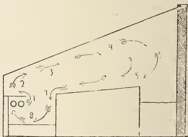
Fig. 3. Section of a Hothouse heated by hot water in the ordinary manner.
