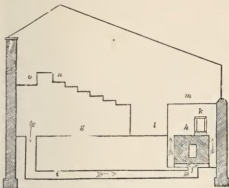
Fig. 133. Section of a greenhouse, with reserve flue and common flue.
