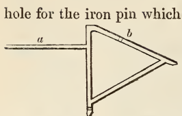
Fig. 114. Iron bracket for supporting a temporary wooden coping.
