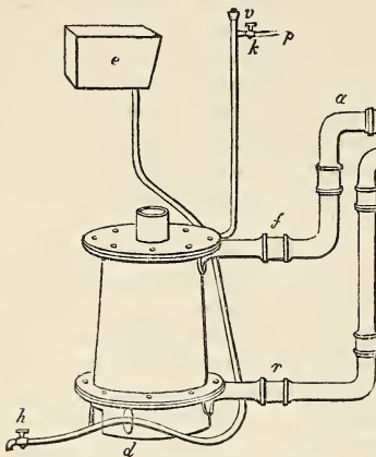
Fig. 150. Rogers's boiler, with the heating-pipe joined to it.
