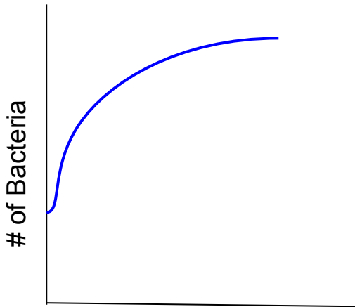
Hours No antibiotics
