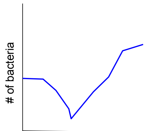
Hours Antibiotics with a population of antibiotic resistant bacteria
