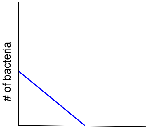
Hours Antibiotics with susceptible bacteria
