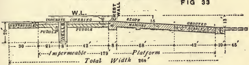
DELTA BARRAGE WEIR
