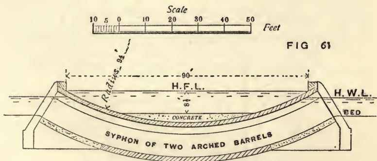
SECTION ALONG AXIS OF BARREL
