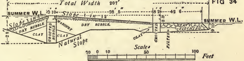
DELTA BARRAGE WEIR
