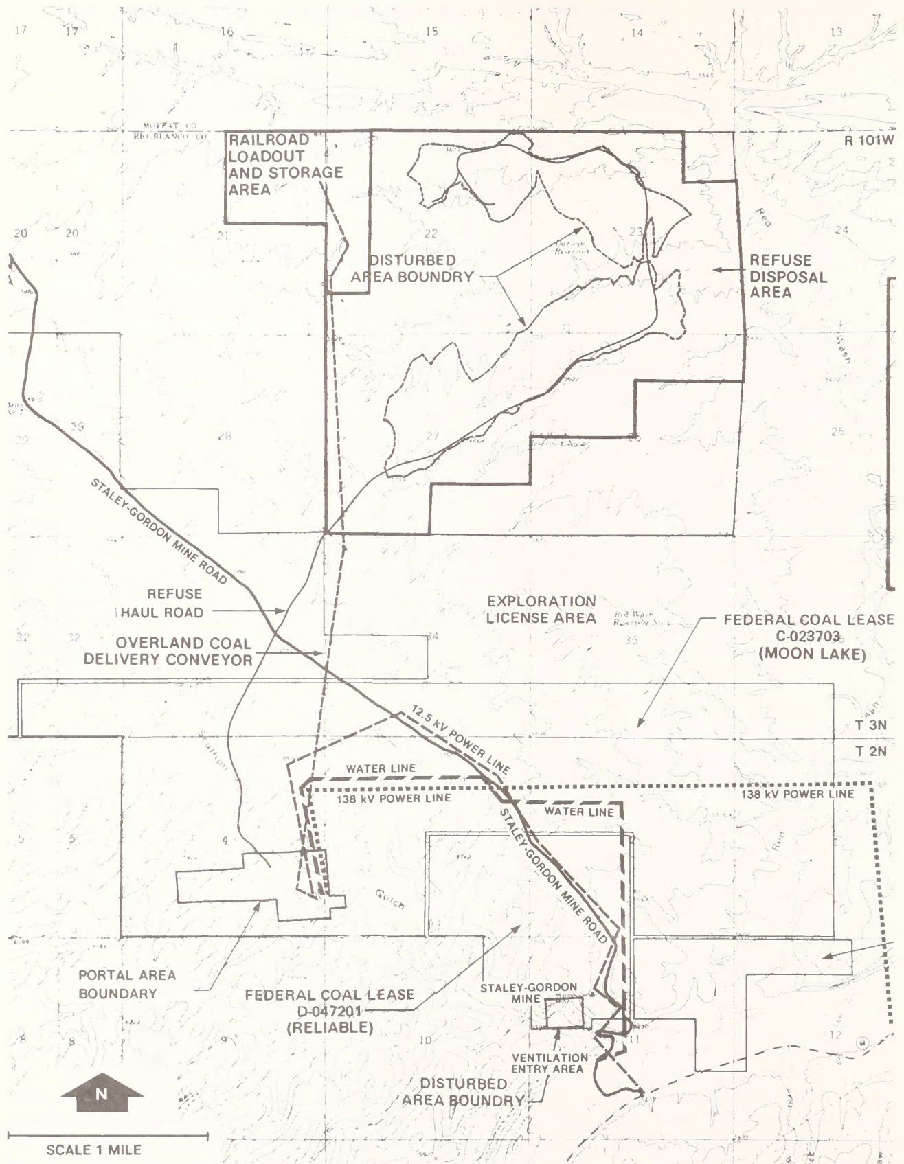
FIGURE 2-13 REFUSE DISPOSAL AREA
