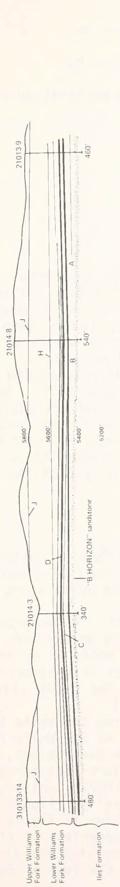
A Typical Cross Section Along the Strike
