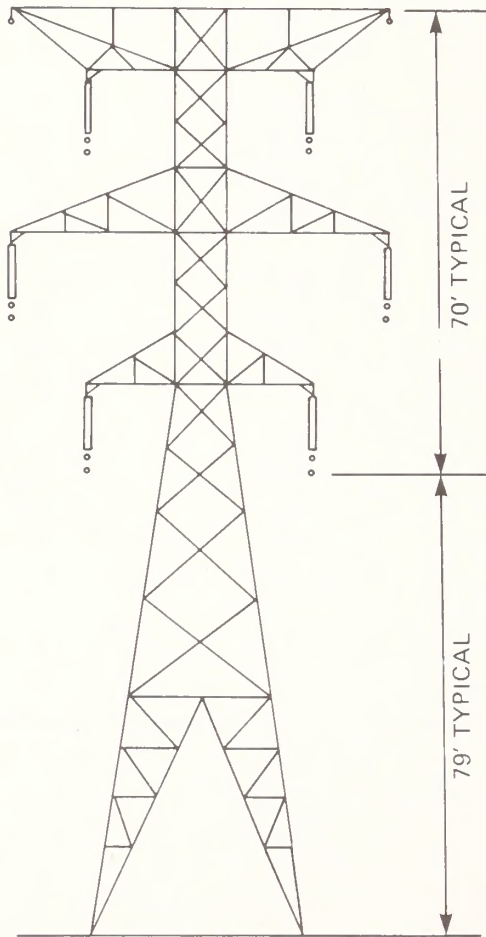
TYPICAL DOUBLE-CIRCUIT 345-kV, 138-kV LATTICE STEEL STRUCTURE
