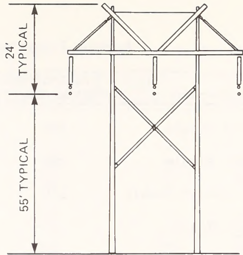
TYPICAL 345-kV WOOD H-FRAME
