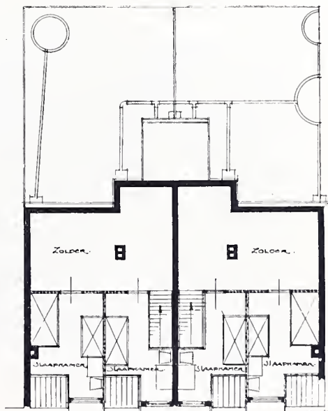
ZOLDERPLAN.
