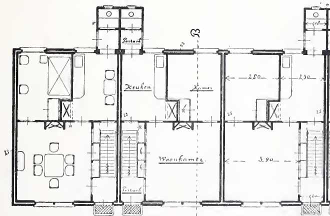
BEGANEGROUND.
