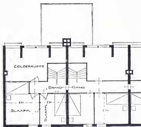
ZOLDERPLAN.
