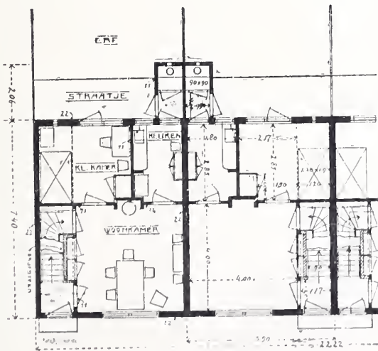
BEGANEGROUND.
