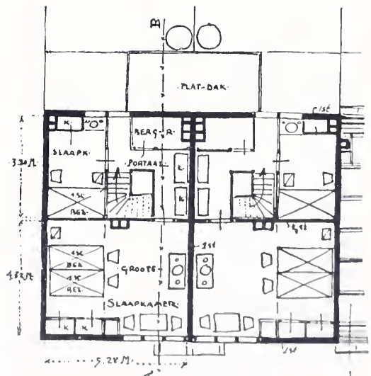
ZOLDERPLAN.
