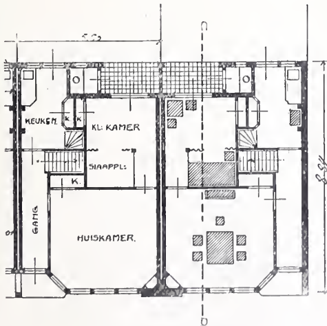
BEGANEGROUND.
