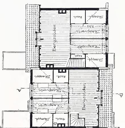
ZOLDERPLAN.
