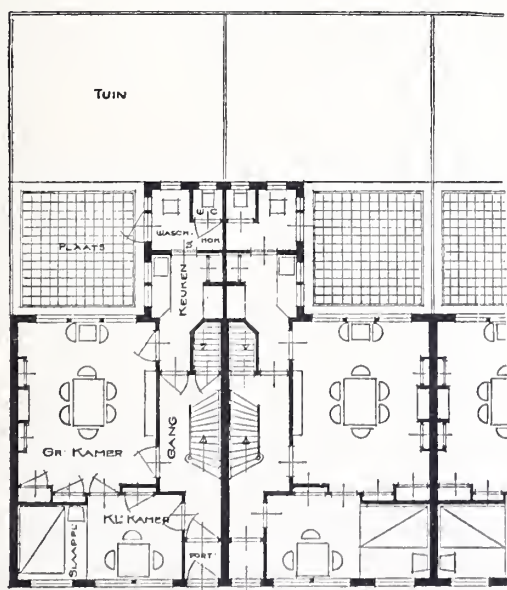
BEGANEGROUND.
