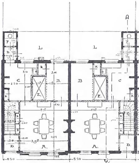
BEGANEGROUND.
