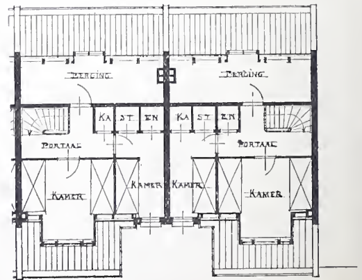
ZOLDERPLAN.
