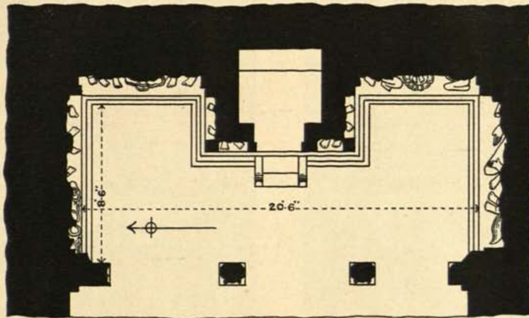
PLAN Scale of 10 5 0 10 20 30 Feet
