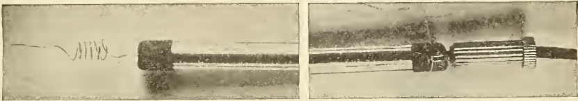
Fig. 534.—Showing terminal and connection of Cushing's electrode ( \frac{3}{4} natural size). Instrument should be 16 inches or more in length.
