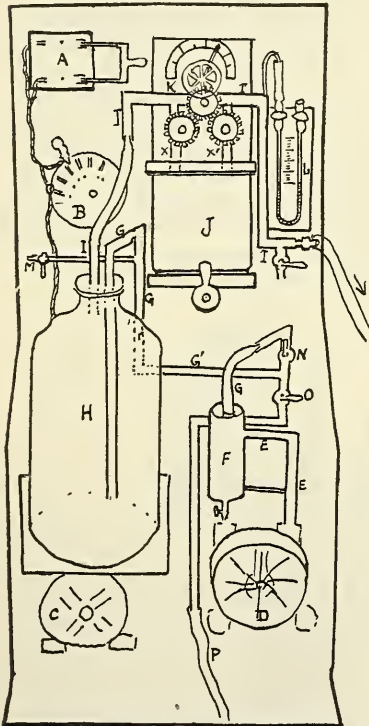
Fig. 570.—Diagram of Elsberg's apparatus showing essential parts.
