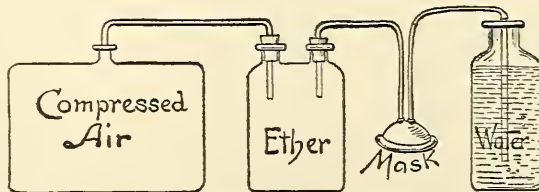
Fig. 569.—Scheme of apparatus for the maintenance of distention of the lung by positive pressure (Robinson and Leland).
