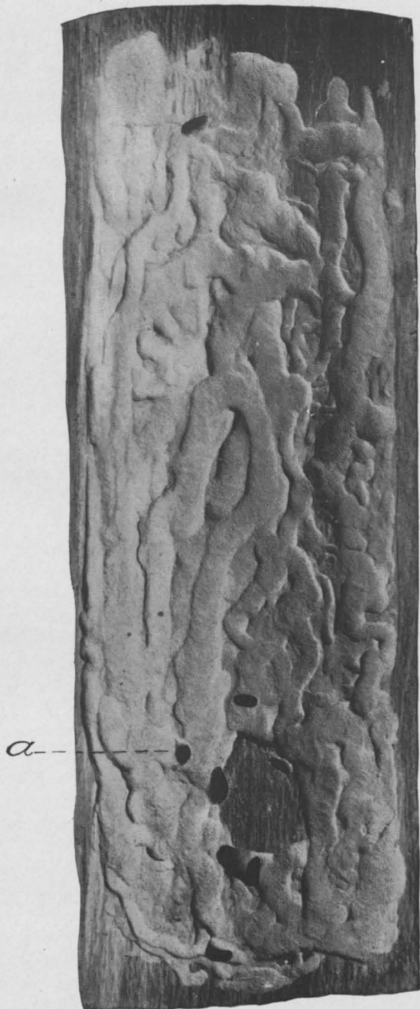
WORK OF THE BLACK-HORNED PINE BORER ( CALLIDIUM ANTENNATUM ).
