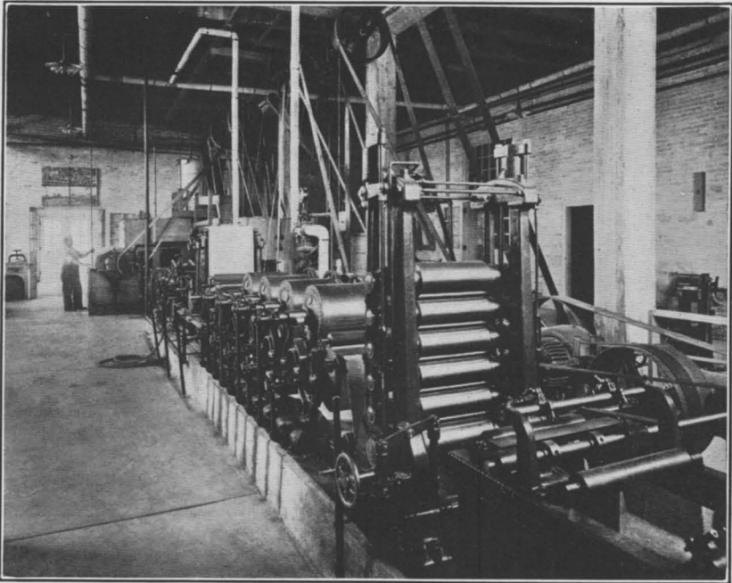
FIG. 1.—PULP AND PAPER LABORATORY, SHOWING FOURDRINIER PAPER MACHINE AND PULP EQUIPMENT.
