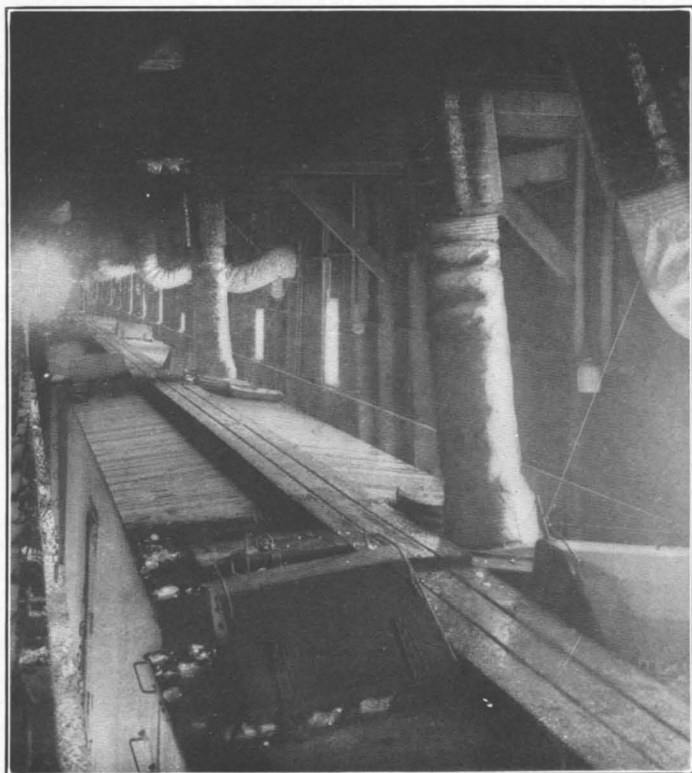
FIG. 2.—INTERIOR OF PRECOOLING SHED, SHOWING FLEXIBLE AIR-PIPE CONNECTIONS FOR WITHDRAWING AIR FROM CARS.
