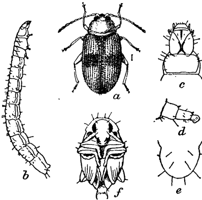
FIG. 3.—The tobacco flea-beetle ( Epicrita parvula ): a, Adult beetle; b, larva, side view; c, head of larva; d, hind leg of same; e, anal segment of same; f, pupa. a, b, f, Enlarged about 15 times; c, d, e, more enlarged. (From Chittenden.)
