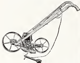
No. 300 DRILL SEEDER
