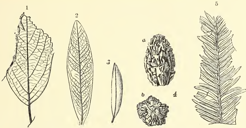
Abb. 8. 1. Parrotia gracilis Heer. 2. Andromeda narbonensis Sap. 3. Ledum limnophilum Ung. 4. Elaeocarpus Albrechti Heer. 5. Taxodium distichum miocenum Heer.
