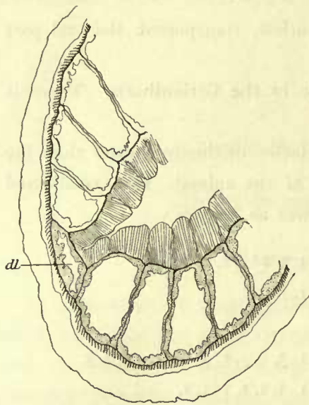
Textfigure 6. Botrucnidifer norvegicus . Transverse section through a portion of the column and stomatodaeum with the mesenteries at the upper part of the stomatodaeum. dl directive chamber.
