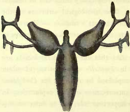
Fig. 7. Dogielia malayana , ca. 40 \mu . From Peda- schenko, who, however, places the animal in the inverted position.
