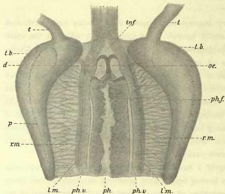
Fig. 11. Pharynx and tentacle-bases of Mertensia ovum . d. diaphragm; inf. infundibulum; l. m. longitudinal muscles; oe. oesophagus; p. series of pigment spots; ph. pharynx; ph. f. pharyngeal (stomodæal) folds; ph. v. pharyngeal vessel; r. m. radial muscles; t. tentacle; t. b. tentacle-basis.
