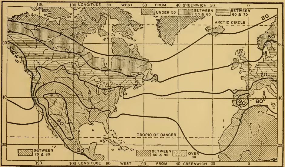
Lines of equal temperature, August
