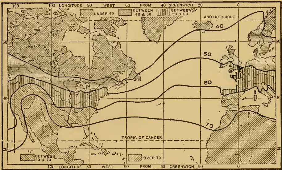
Lines of equal temperature. annual
