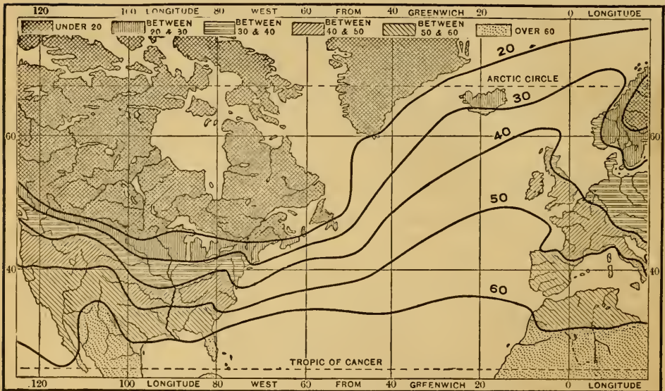
Lines of equal temperature, February
