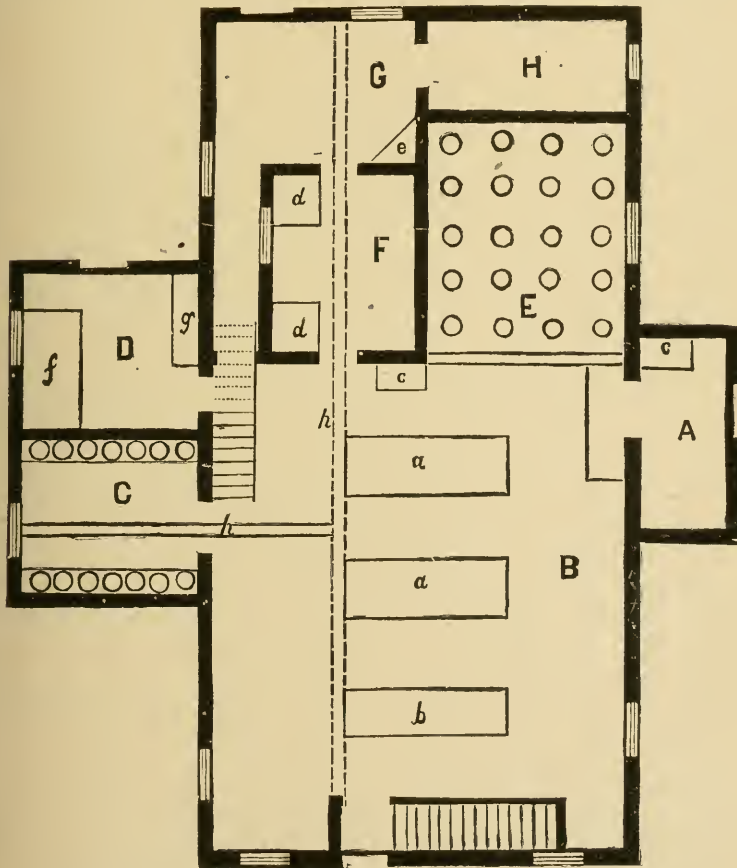
GROUND PLAN OF COMBINED CREAMERY AND CHEESE FACTORY.
