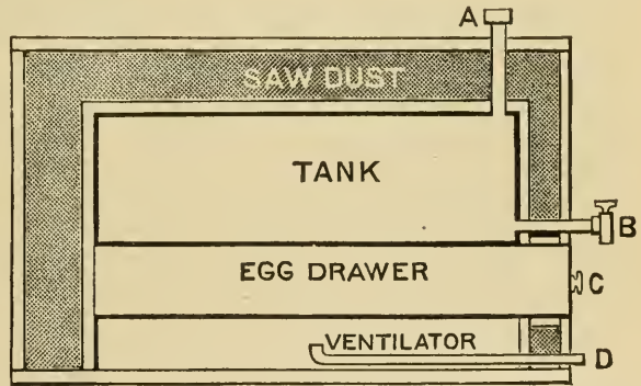
FIG. 6. SECTIONAL VIEW OF INCUBATOR.
