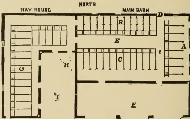
MAIN FLOOR OF BARN.
