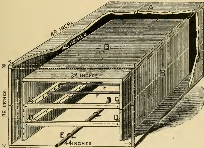
FIGURE 2. INTERIOR OF INCUBATOR.
