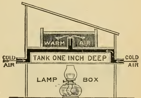
FIG. 2. SECTIONAL VIEW.
