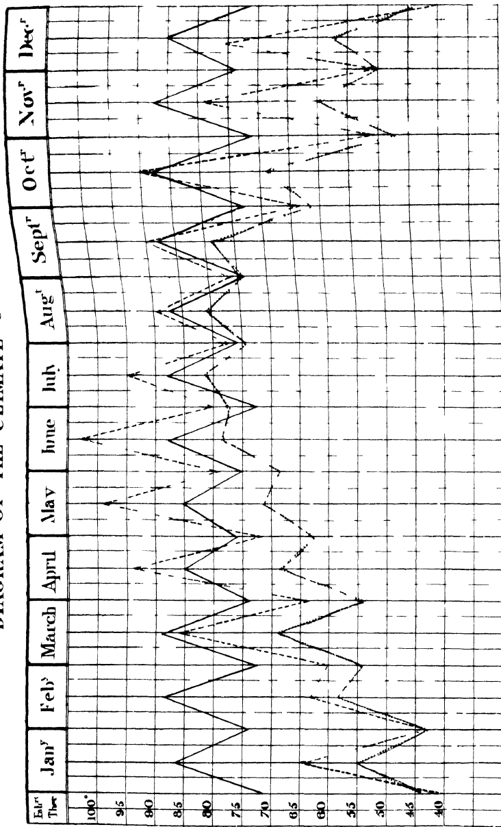
DIAGRAM OF THE CLIMATE OF INDIA.
